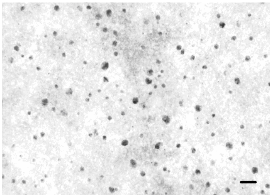
Fig. 3. TEM Photograph of Dextran-Protoporphyrin Nanoparticles (10 kDa). Scale bar: 20 nm.
