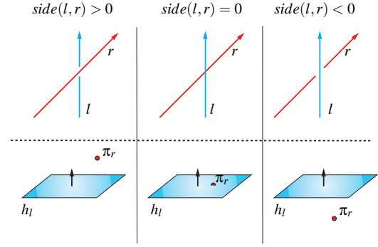
Figure 1: Above: The relative orientation of two lines is given by the sign of the side operator. Under: Since side(l, r) = h_l(\pi_r) , applying the side operator comes down to testing the position of the Plücker point of one line against the dual hyperplane of the other line
