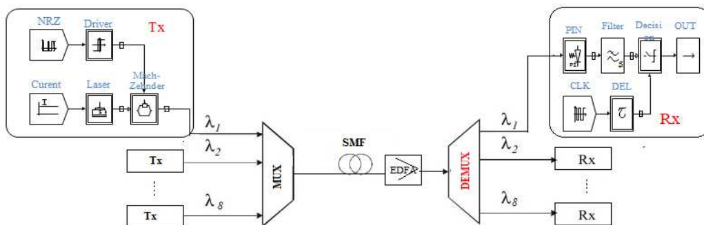
Figure 1. Configuration of the simulated link.
