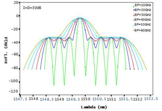
Figure 2. Transfer function for different values of BP.
