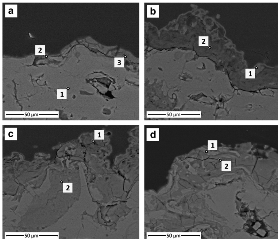
Fig. 8. Cross section of the coatings after immersion in SBF: (a) APS-HA coating after 1 day in SBF; (b) APS-HA/SPS-BG-Ca coating after 1 day in SBF; (c) APS-HA/SPS-BG-Ca coating after 7 days in SBF; (d) APS-HA coating after 14 days in SBF.
