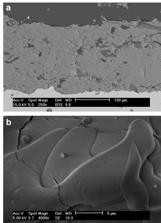
Fig. 4. APS-HA coatings: (a) cross section, (b) surface.
