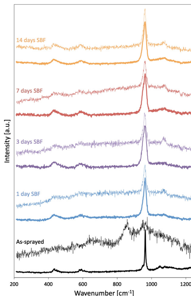
Fig. 10. Evolution of the Raman spectra of the APS-HA samples (bold trace) and of those of the APS-HA/SPS-BG_Ca samples (thin trace) after in vitro tests. The spectra of the as-sprayed samples are included as a term of comparison.
