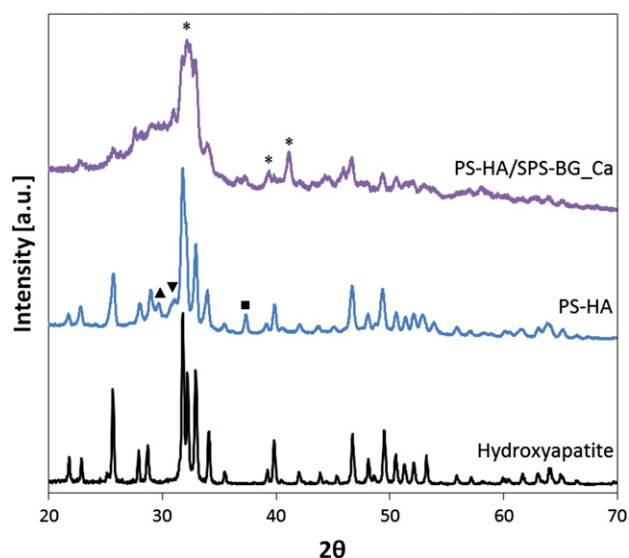
Fig. 3. Comparison between the X-ray diffraction pattern of the commercial HA feedstock powder and those of the coatings. Symbols: *, larnite ( \text{Ca}_2\text{SiO}_4 , 01-070-0388); ▲, TTCP (00-025-1137); ▼, TCP (00-009-0169); ■, CaO (01-075-0264); the peaks without symbol are due to HA (01-089-6437).
