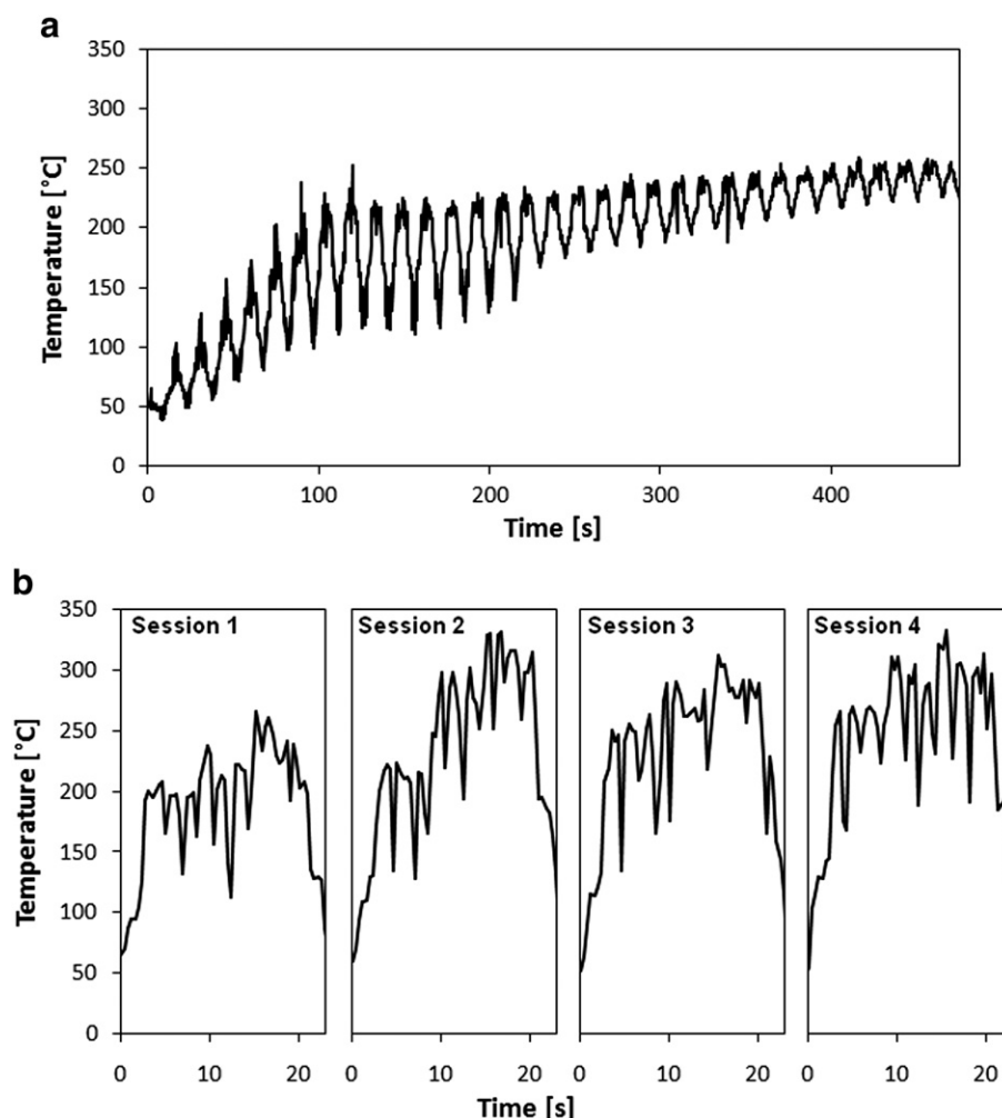
Fig. 2. Substrate temperature measured during spray sessions: (a) atmospheric plasma spray deposition of HA, (b) suspension plasma spray deposition of BG_Ca.
