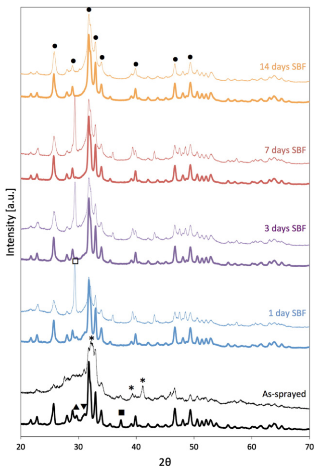
Fig. 9. Evolution of the XRD spectra of the APS-HA samples (bold trace) and of those of the APS-HA/SPS-BG_Ca samples (thin trace) after in vitro tests. The spectra of the as-sprayed samples are included as a term of comparison. Symbols: *, larnite ( \text{Ca}_2\text{SiO}_4 ); ▲, TCP; ▼, TCP; ■, CaO; □, \text{CaCO}_3 ; ●, HCA. The peaks without symbol are due to HA.
