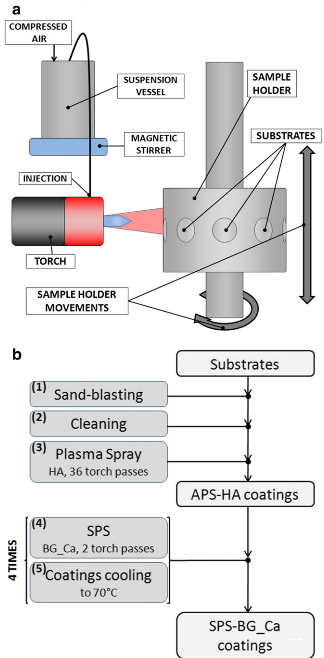
Fig. 1. Coatings' deposition process: (a) SPS set-up, (b) production scheme of the coatings.
