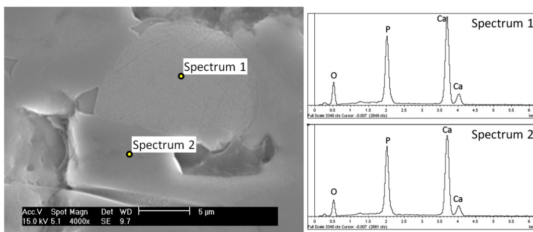
Fig. 5. Details of the APS-HA cross section and corresponding EDS microanalyses.
