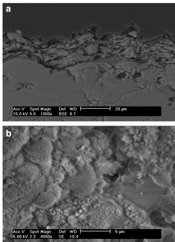
Fig. 6. APS-HA/SPS-BG_Ca coatings: (a) cross section; (b) surface.
