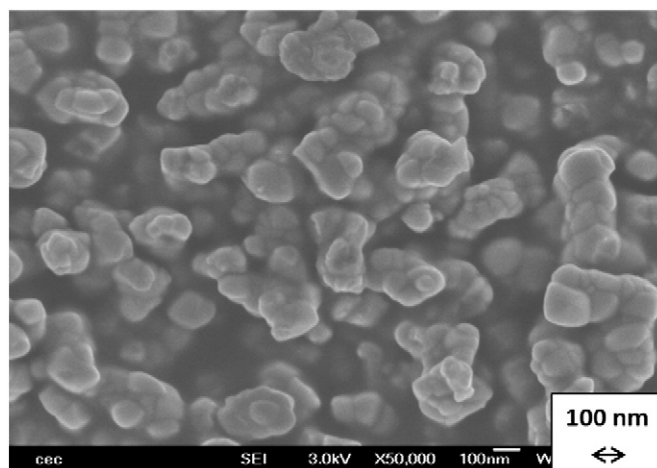
Fig. 2. FE-SEM micrograph (secondary electrons) of Tosoh powder.
