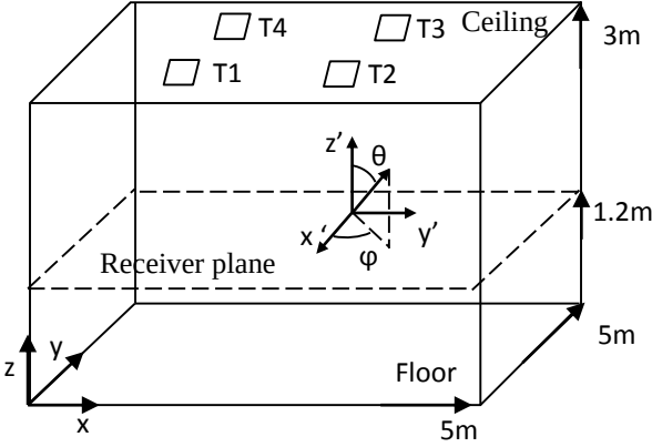
Fig. 1. VLC scenario configuration
