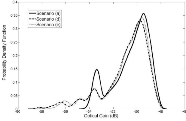
Fig. 5. Probability density function of the optical gain for scenarios (a), (d) and (e)
