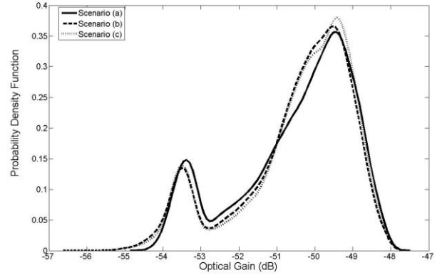
Fig. 4. Probability density function of the optical gain for scenarios (a), (b) and (c)
