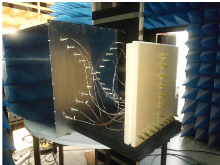
Figure 6. 'T' shaped antenna array connected to the metallic microwave cavity.
