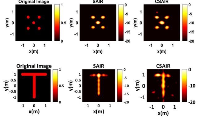
Figure 4. Simulation results of point-like sources and a 'T' shaped 2-D source imaging with conventional SAIR and CSAIR imaging system.
