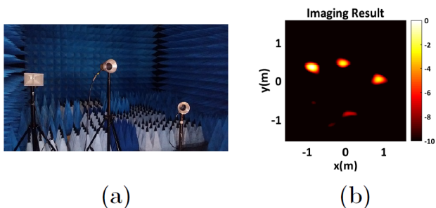
Figure 7. Imaging Results. (a) Three horn antennas used in the noise source emulator. (b) Imaging result of the noise sources.
