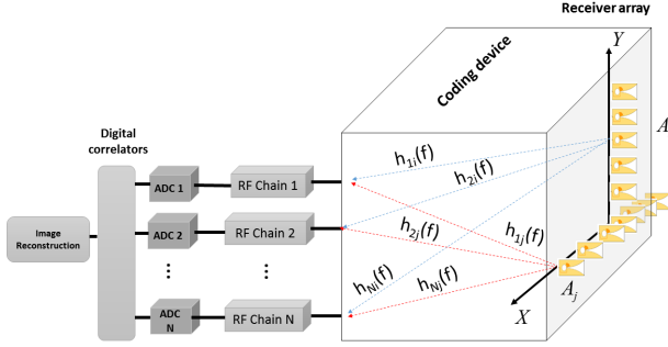
Figure 2. Passive coded SAIR architecture. M received signals are coded into N measured signals.
