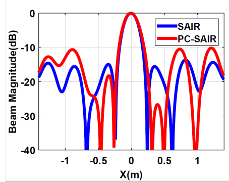
Figure 5. Cut-plane along X-axis of the point-like sources image.
