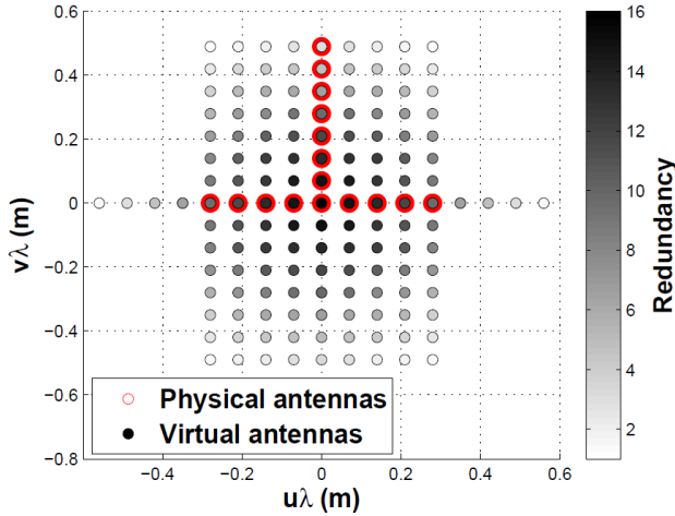
Figure 3. T-shaped antenna array and the corresponding (u, v) coverage.
