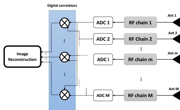
Figure 1. Architecture of a conventional microwave radiometer.
