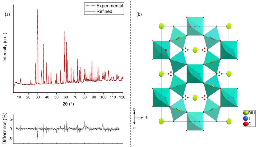
Fig. 5: (a) Final profile for the refinement of the LBT compound and (b) Representation of the pyrochlore \text{Li}_{0.38}\text{Bi}_{1.62}\text{Ti}_2\text{O}_6\text{O}'_{0.89} structure in the \text{Fd}\bar{3}\text{m} space group (color online)
