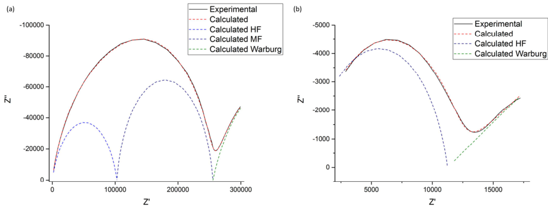
Fig. 7: Examples of two refined Nyquist diagrams: (a) at 325°C (low temperature range and (b) 550°C (high temperature range) (color online)
