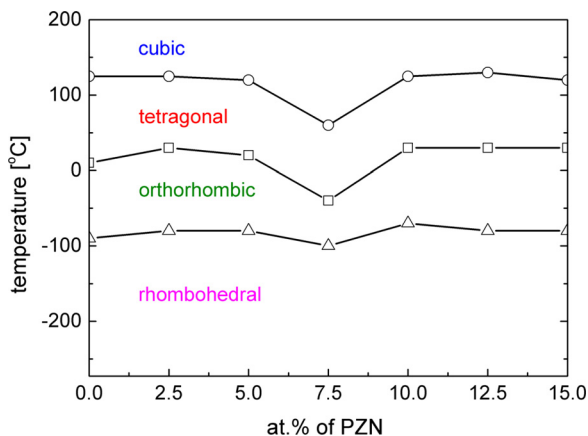
FIG. 3. Phase diagram of (1-x)\text{BT}-x\text{PZN} ceramics.
