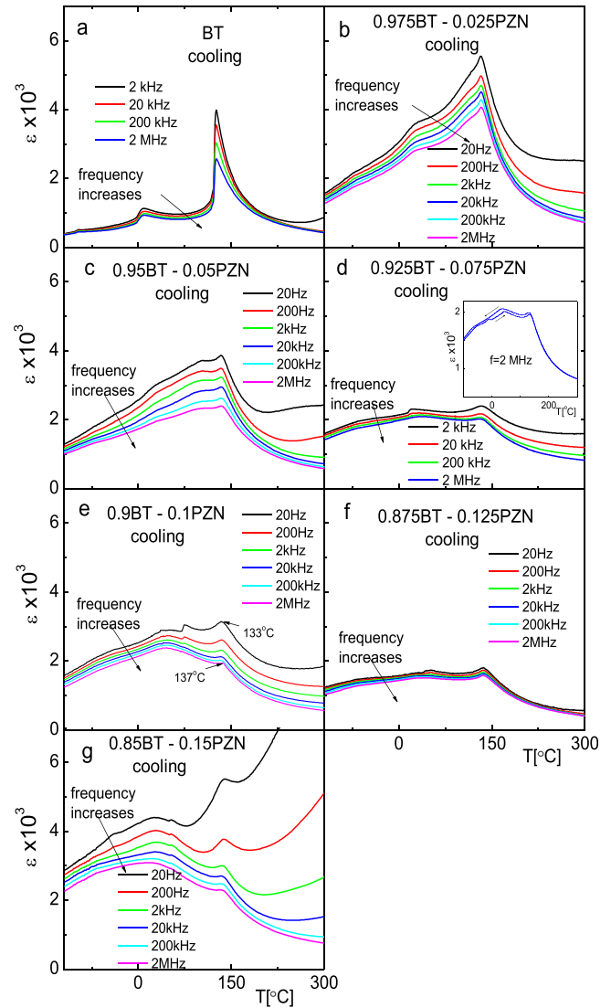
FIG. 4. Temperature dependence of the electric permittivity \epsilon of (1-x)\text{BT}-x\text{PZN} ceramics on cooling.
