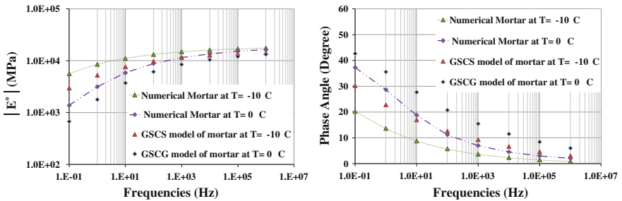
Fig. 4 Numerical and analytical phase angle and master curves of mortar at T = -10^\circ\text{C} and T = 0^\circ\text{C}
