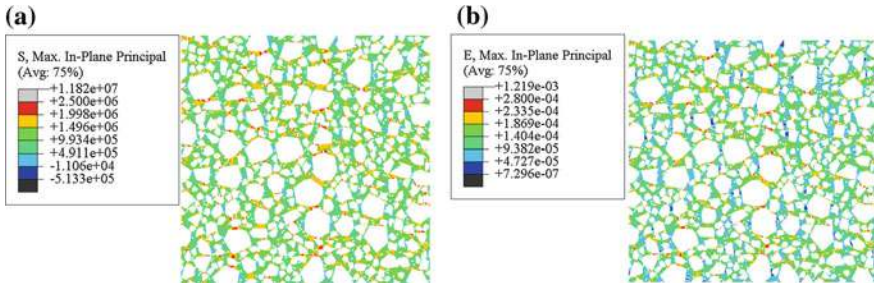
Fig. 6 Distribution of stress and strain within a heterogeneous model
