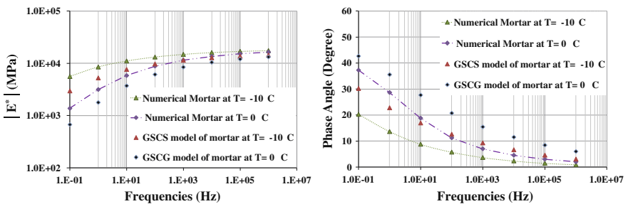
Fig. 4 Numerical and analytical phase angle and master curves of mortar at T = -10\text{ }^\circ\text{C} and T = 0\text{ }^\circ\text{C}
