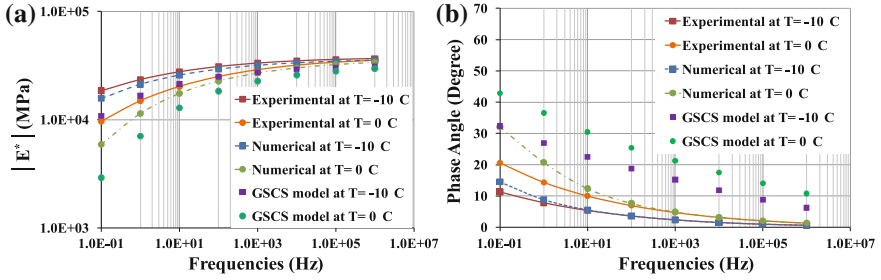
Fig. 5 Numerical and analytical phase angle and master curves of asphalt mixture compared to experimental one at T = -10^\circ\text{C} and T = 0^\circ\text{C}
