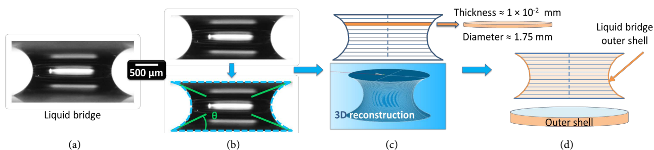
Figure 5. Water liquid bridge volume and area evaluation in the case of a hydrophilic contact: (a) liquid bridge of deionized water; (b) cropped image, edge detection (dashed line) and evaluation of the four contact angles; (c) liquid bridge volume evaluation (gravity center in dashed line) and three-dimensional reconstruction; (d) liquid bridge outer shell evaluation (exchange surface). The same operation is realized on hydrophobic contacts.
