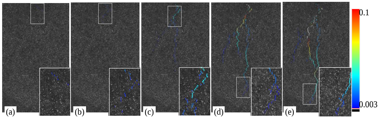
Figure 9. 2P-DIC crack opening by plotting \varepsilon for \varepsilon_s=0.003 , subset size 64x8 pixels.
