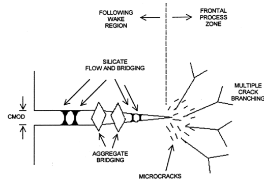
Figure 2: Schematic representation of the crack propagation zone for refractories [4]
