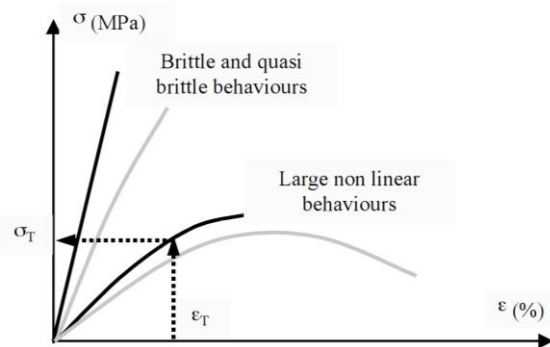
Figure 1: Typical stress/strain behaviours observed in tension on refractory materials [3]
