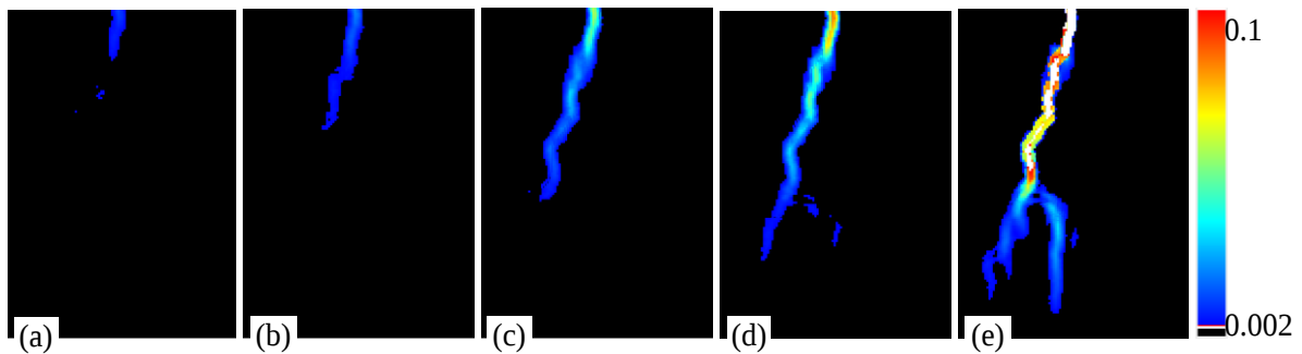
Figure 6. Standard DIC horizontal strain field with \epsilon_s=0.002 , subset size 32x32 pixels, subset shift 8 pixels, strain gauge length 32 pixels
