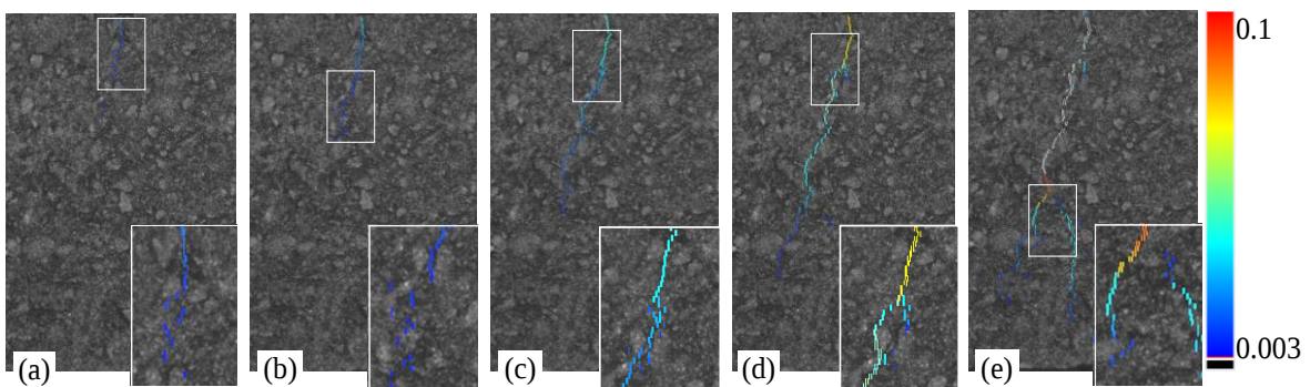
Figure 7. 2P-DIC crack opening by plotting \epsilon for \epsilon_s=0.003 , subset size 64x8 pixels.
