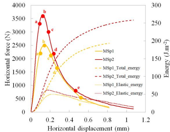
Figure 5. Horizontal load and energies versus horizontal load displacement for MSp1 and MSp2
