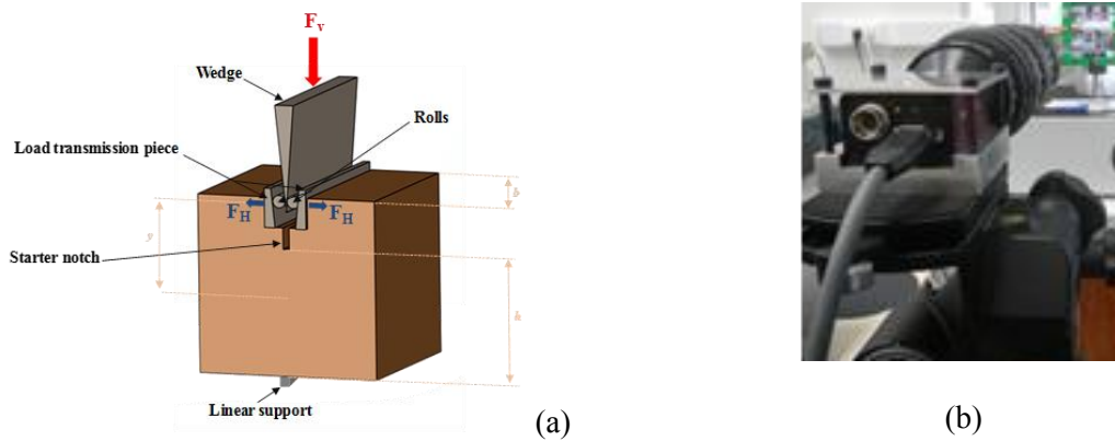
Figure 3: Principle of wedge splitting test with sample's geometry (a) and image acquisition setup (b)
