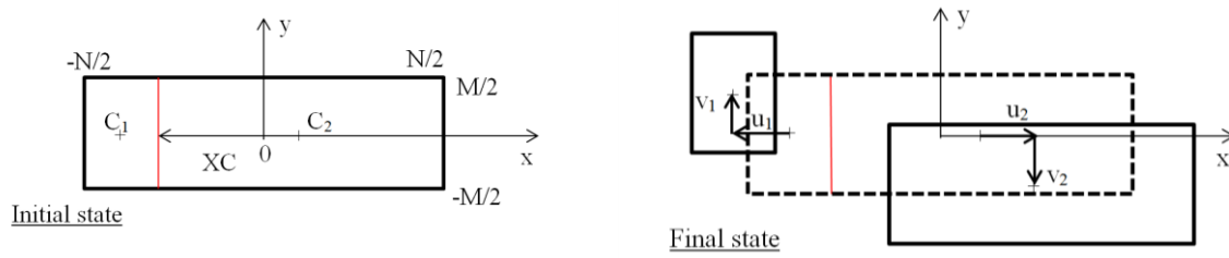
Figure 4. Principle of the 2P-DIC, decomposition of a subset.
