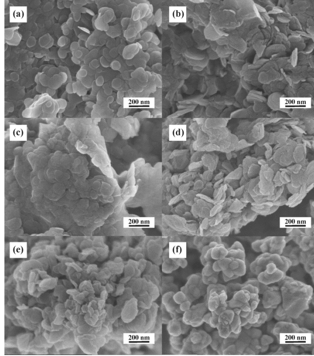
Figure 2: FE-SEM images of (a) LDH-NO 3 , (b)LDH-IBU(10:1), (c)LDH-IBU(8:1), (d)LDH-IBU(6:1), (e)LDH-IBU(4:1), (f)LDH-IBU(2:1).
