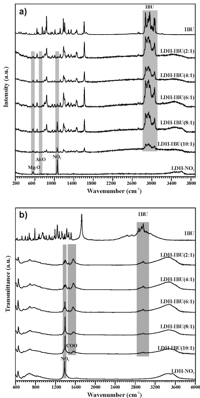
Figure 3: (a) Raman spectra (b) FTIR spectra of IBU, LDH-NO 3 , LDH-IBU(2:1), LDH-IBU(4:1), LDH-IBU(6:1), LDH-IBU(8:1), LDH-IBU(10:1).
