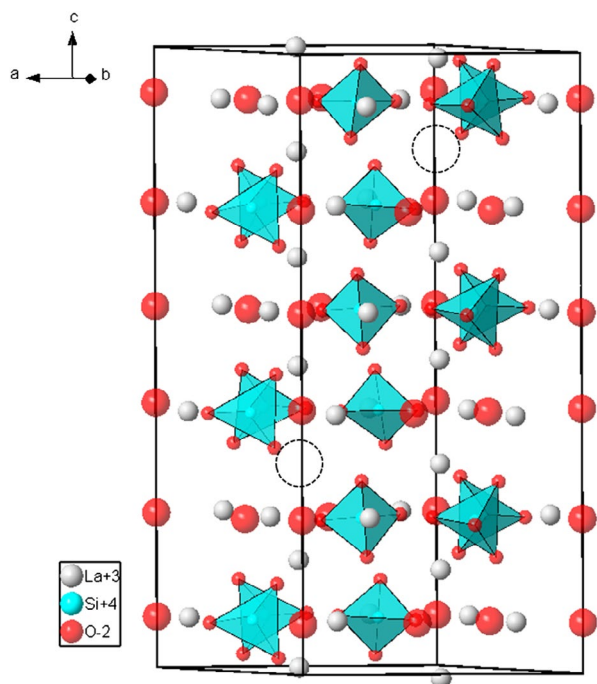
Figure 2. DFT-relaxed (1×1×3) supercell of the \text{La}_{9.33}(\text{SiO}_4)_6\text{O}_2 model (M1) used in this study. The empty broken-line circles indicate positions of La1 vacancies.
