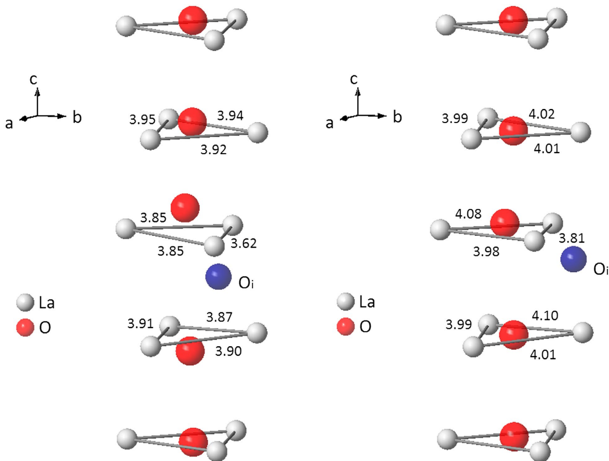
Figure 7. Perspective views of the conduction channel, showing the O4 oxide ions, the La2 lanthanum triangles, the Oi interstitial oxide ion and some triangle edge lengths for model M2 (left image) and model M3 (right image).
