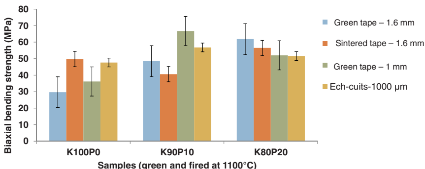
Figure 5. Biaxial flexural strength of some green and sintered (1100°C) kaolin-palygorskite samples. For each series from left to right: green tape 1.6 mm; sintered tape 1.6 mm; green tape 1 mm and sintered tape 1 mm
