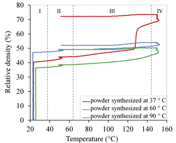
Fig. 5. Relative density changes of samples during SPS.
