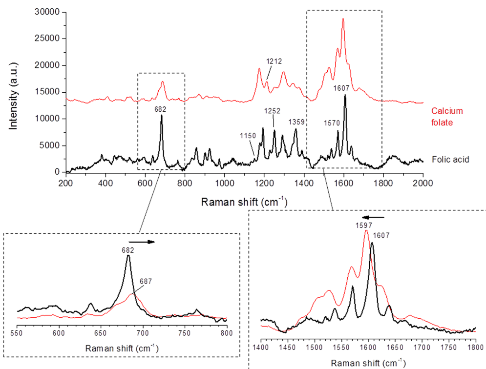
Figure 5. Raman spectra for pure FA and precipitated calcium folate.
