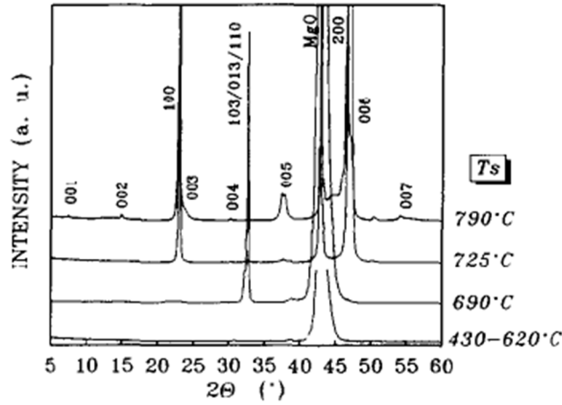
Fig. 1. X-ray diffraction patterns of YBaCuO films on MgO as functions of the substrate temperature.
