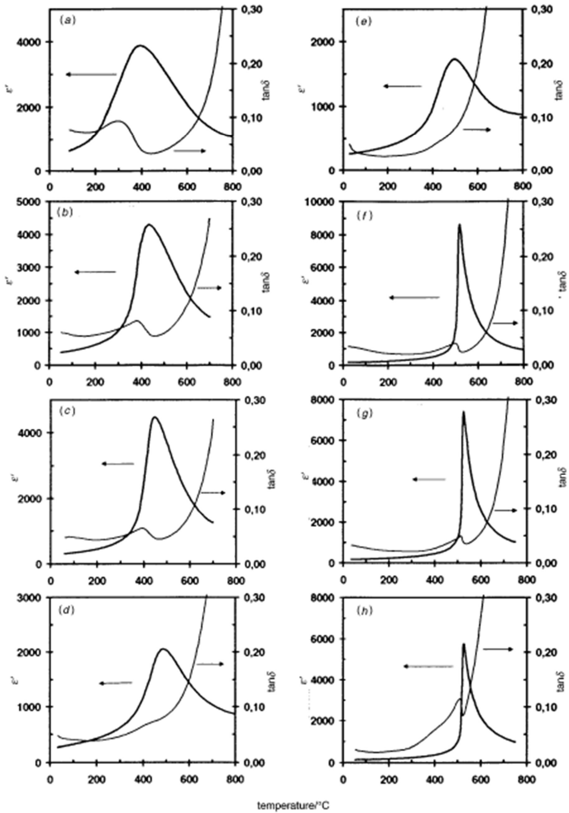
Fig. 7 KBT-PT system. Permittivity and loss vs. temperature for (K_{0.5}Bi_{0.5})_{0.5-1-x}Pb_xTiO_3 : x = 0 (a), 0.09 (b), 0.18 (c), 0.30 (d), 0.40 (e), 0.50 (f), 0.60 (g) and 0.80 (h).
