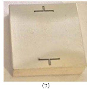
Fig. 1. Parallelepipedic dielectric resonator made of zirconia. (a) CAD model, (b) prototype.
