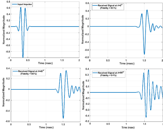
Fig. 4. Normalized input and received signals by virtual probes for varying angles in the E-plane.
