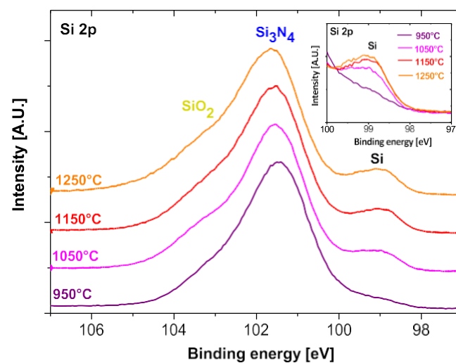
Figure 6. XPS Si 2p spectra obtained on samples pyrolyzed at different temperatures.
