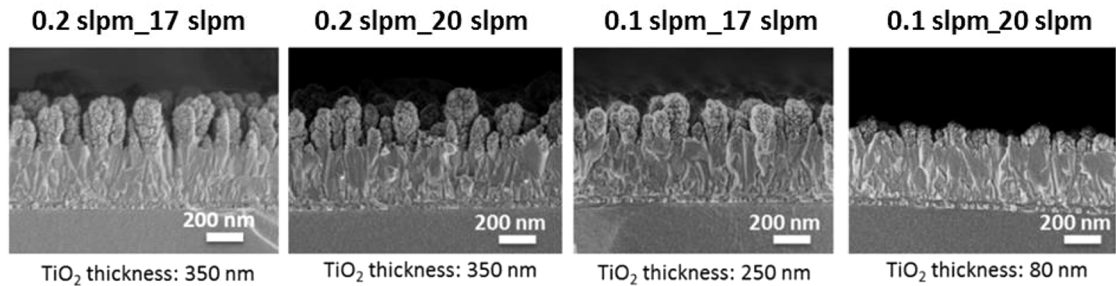
Fig. 4. FESEM images of films elaborated with the different gas flow rates combinations ([TTIP flow rate]_[Ar plasma flow rate]) on glass/FTO substrates, from the plasma phase with the higher TTIP proportion (left) to the lower proportion.
