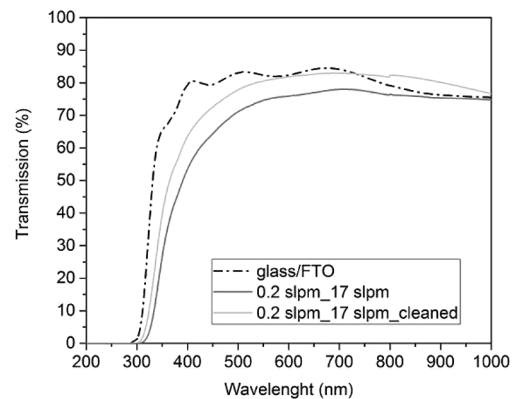
Fig. 6. UV-Visible transmission results after cleaning the 0.2 slpm_17 slpm titania film.
