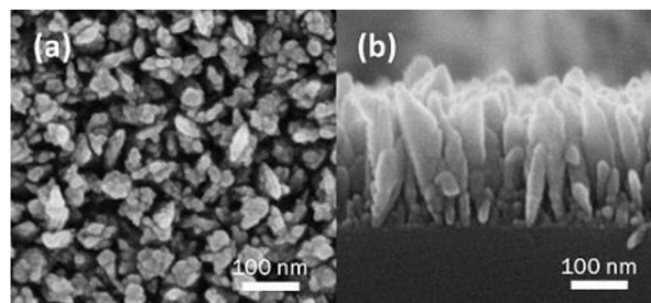
Fig. 2. FESEM images of the optimized TiO 2 thin film on a silicon wafer, (a) top view and (b) cross-section.
