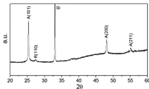
Fig. 3. XRD pattern of the titania film elaborated in the optimized conditions.
