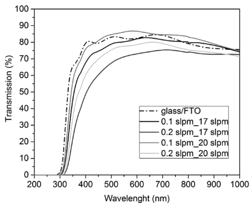
Fig. 5. UV-Visible transmission results.
