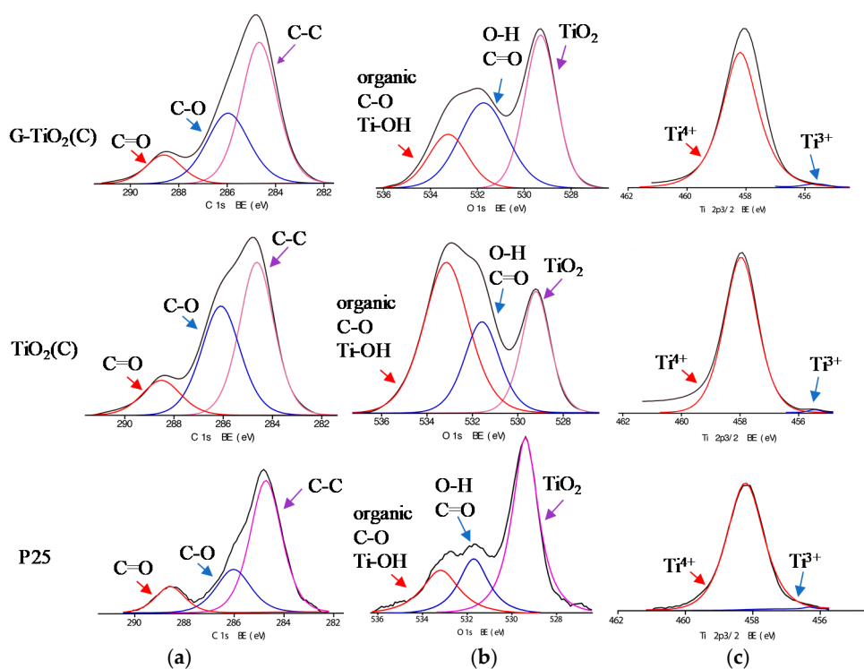
Figure 6. XPS data for G-TiO 2 (C) (top) and TiO 2 (C) (middle) and P25 (bottom) samples for: (a) C 1s, (b) O 1s and (c) Ti 2p 3/2 .
