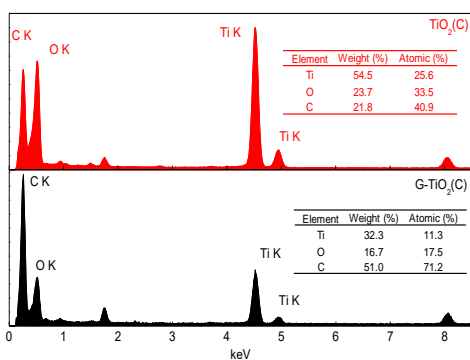
Figure 7. EDS data for TiO 2 (C) (red, upper) and for G-TiO 2 (C) (black, down).
