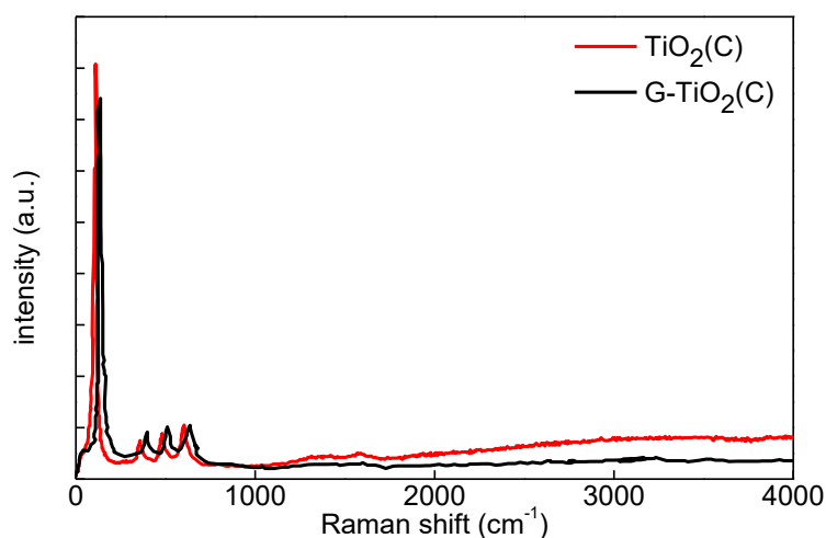
Figure 5. Raman spectra of TiO 2 (C) (red) and G-TiO 2 (C) (black).
