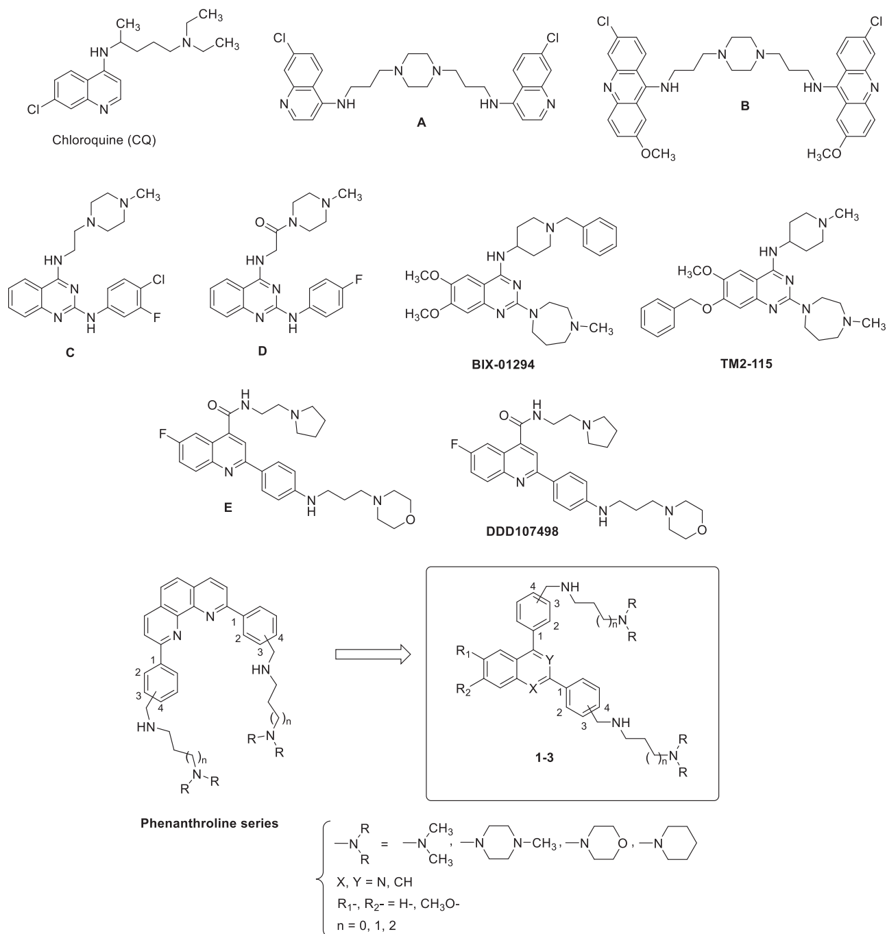
Figure 1. The structures of chloroquine (CQ), bisquinoline A, bisacridine B, 2-anilino-4-aminoquinazolinones C, D, diaminoquinazolinones BIX-01294 and TM2-115, and quinolinones E and DDD107498, and newly synthesised 2,4-bis[(substituted-aminomethyl)phenyl]quinoline, 1,3-bis[(substituted-aminomethyl)phenyl]isoquinoline and 2,4-bis[(substituted-aminomethyl)phenyl]quinazolinone derivatives 1–3.
