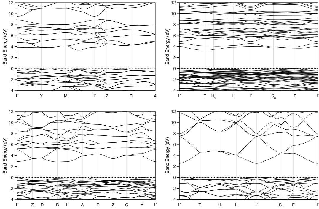
Figure 2. Electronic bandstructures (from top to bottom) of \alpha - \text{TeO}_2 , \text{Te}_4\text{O}_9 , \text{Te}_2\text{O}_5 , and \beta - \text{TeO}_3
