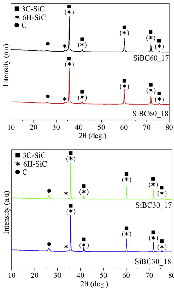
Fig. 3. XRD patterns of the sintered samples.
