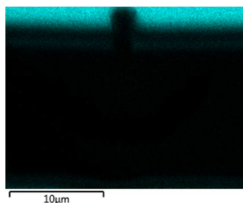
Figure 10- SEM observation and chemical composition map analysis of a cross-section obtained on a 2.5 \mu\text{m} diameter artificial defect produced using FIB and after “in situ electrochemical test”
