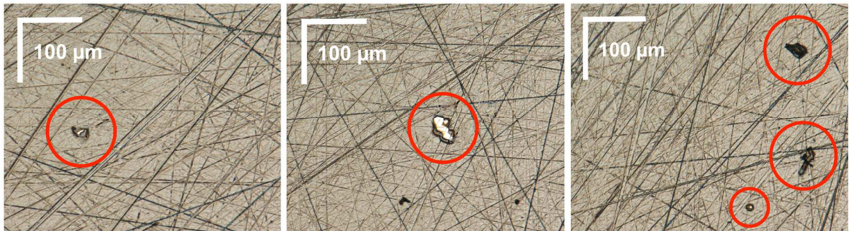
Figure 2- Typical defects due to the presence of dusts particles (substrate roughness Ra = 0.05 \mu m )
