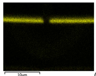
Figure 10- SEM observation and chemical composition map analysis of a cross-section obtained on a 2.5 \mu\text{m} diameter artificial defect produced using FIB and after “in situ electrochemical test”
