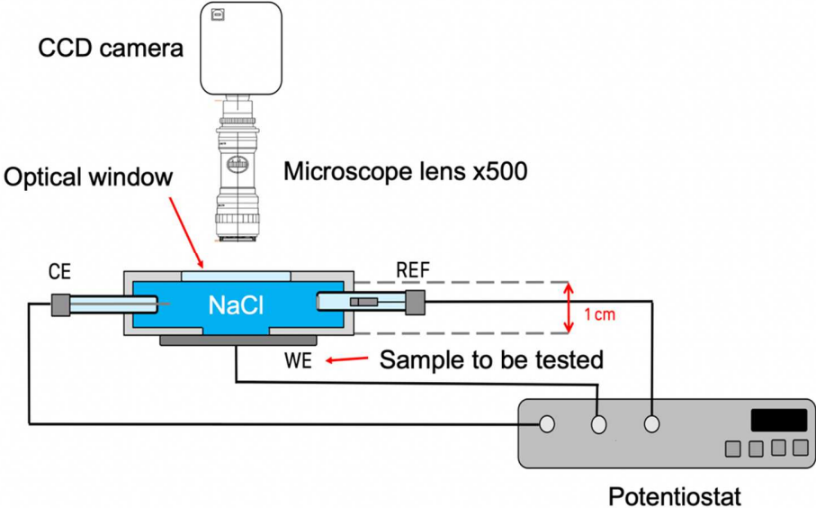
Figure 1- Schematic diagram of the set up for the “in situ electrochemical test”; CE = platinum counter electrode, WE = working electrode and REF = saturated calomel reference electrode
