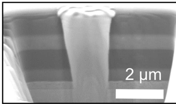
Figure 7- SEM top surface(a) and cross-sectional (b) views of a 2.5 \mu\text{m} diameter artificial defect produced by FIB machining.
