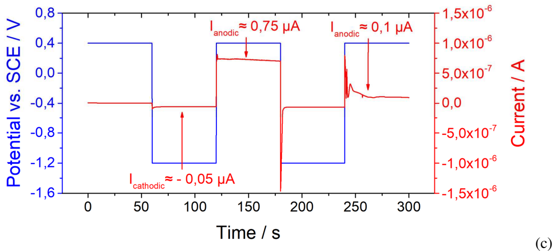
Figure 8- Electrochemical activation of an artificial defect
