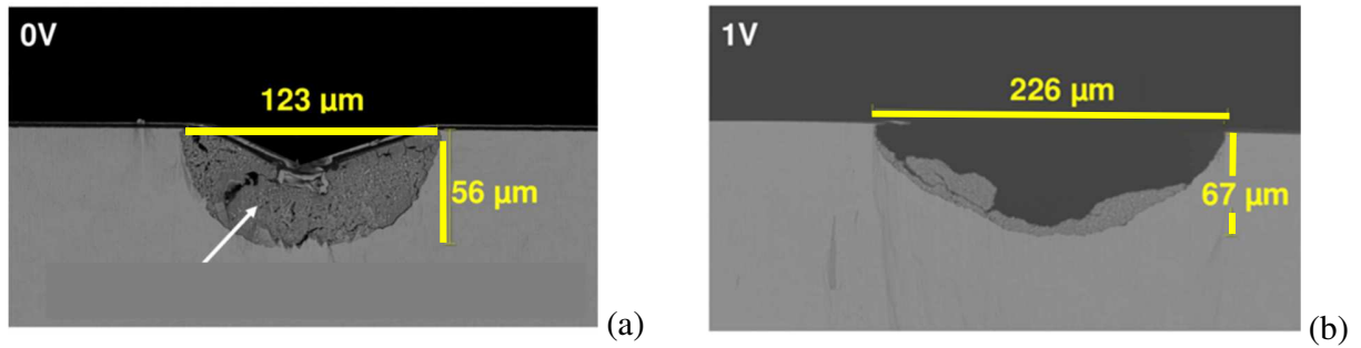
Figure 5- SEM cross-sections of corrosion attack triggered by an isolated defect.
