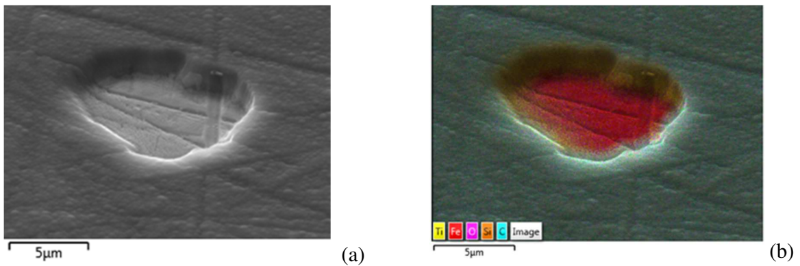
Figure 3- (a) SEM and (b) chemical analysis (EDAX) of the surface of a 10 \mu m diameter defect in a DLC coating (same conditions than in Table 1).
