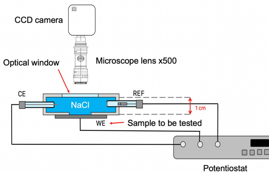
Figure 1- Schematic diagram of the set up for the “in situ electrochemical test”; CE = platinum counter electrode, WE = working electrode and REF = saturated calomel reference electrode
