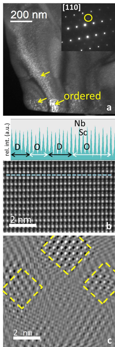
Fig. 4 a) TEM – DF image of MA1000 grain with the corresponding SAED pattern in [110] zone axis. Ordered areas within the grain are marked with arrows. A weak and diffuse (\frac{1}{2} \frac{1}{2} \frac{1}{2}) superstructure reflection is marked with a circle, b) HAADF-STEM image with the corresponding intensity profile of B site ions (O, D-ordered/disordered area); the dotted line represents the area where the intensity profile was performed. c) Inverse FFT image from superstructure reflections with marked B-site ordered areas.
