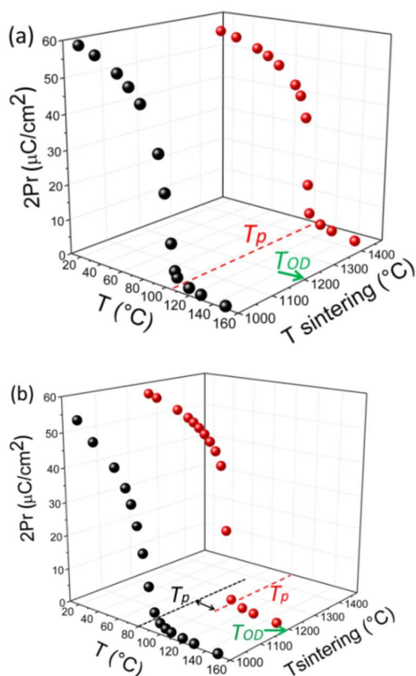
Fig. 7 Temperature dependence of 2P_r for (a) MA1000, MA1420q and (b) SS1000, SS1200. The sintering temperature of ceramics is shown in y axis. The T_{OD} from the literature [3, 4] is marked by an arrow. In (a) the dashed horizontal lines represent the T_p of MA1000 and MA1420q ceramics. In (b) the red dashed horizontal line represents the T_p for SS1200. The dark dotted horizontal line represents the T_p for SS1000. The black arrow marks the difference of \sim 20 °C between these two temperatures.
