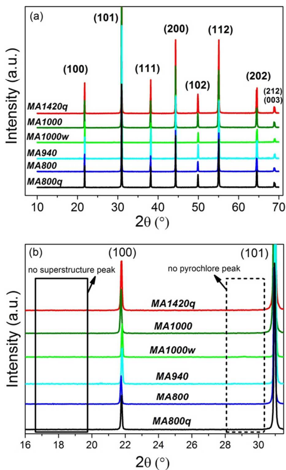
Fig. 2 (a) Room-temperature XRD spectra (PANalyticalX'Pert PRO MPD using the Cu-K \alpha_1 radiation) of the PSN ceramics exposed to different thermal treatments as described in Table 1. The indexed peaks of the perovskite phase are shown in brackets (ICSD #80922). (b) Zoom of the XRD spectra from 16 to 31.5° showing that there is no secondary-phase (dashed box) or superstructure peaks (solid box).
