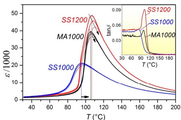
Fig. 6 The \epsilon - T at 1, 10 and 100 kHz and (inset) \tan \delta vs. temperature at 10 kHz for MA1000, SS1000 and SS1200.
