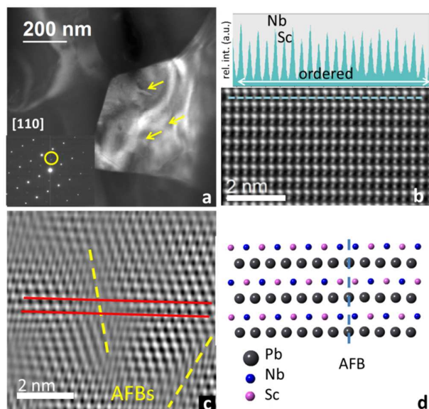
Fig. 5 a) TEM – DF image of SS1000 ceramic grain with the corresponding SAED pattern in [110] zone axis. Between ordered regions antiphase boundaries (AFBs) were observed (labelled with arrows) as also by Perrin et al [9]. The superstructure reflection at (\frac{1}{2} \frac{1}{2} \frac{1}{2}) is marked with a circle, b) HAADF-STEM image with the corresponding intensity profile of B site ions, with alternating Nb/Sc intensities. The dotted line represents the area where the intensity profile was performed c) inverse FFT image from superstructure reflections with marked AFB. Two red parallel lines indicate the change in B-site contrast intensity, d) model of ordered PSN structure showing the AFB.
