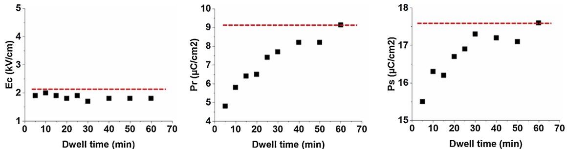
Fig. 4. Ferroelectric properties measured at 3 kV/mm for samples sintered by MWS with different dwell times (the dashed lines show values obtained for the CS sample).
