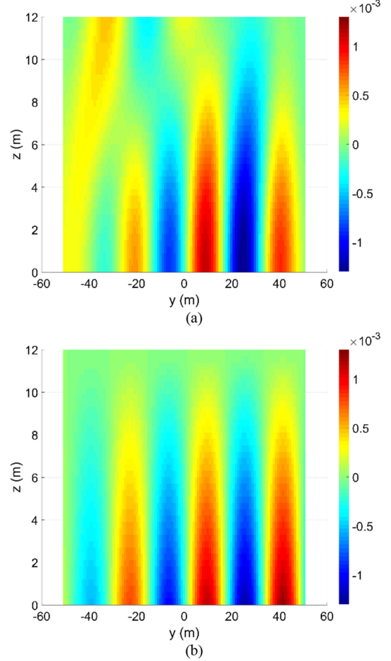
Fig. 8. Field charts of the \text{Real}(H_y) component in the lateral face yz_{\text{front}} at f = 15.37 MHz and \phi_i = 30^\circ . (a) Original chart. (b) Interpolated chart.
