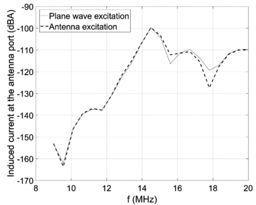
Fig. 13. Magnitude of the induced current computed with plane wave and antenna excitation, for incidence angle \phi_i = 45^\circ .
