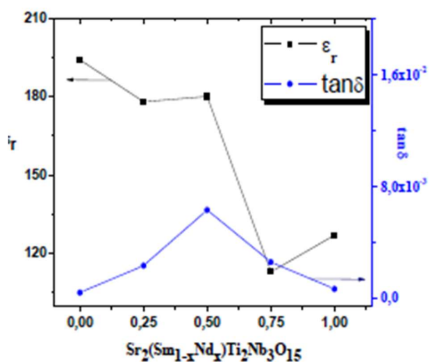
Fig. 10: Variation of \epsilon_r and \tan(\delta) with composition x.
