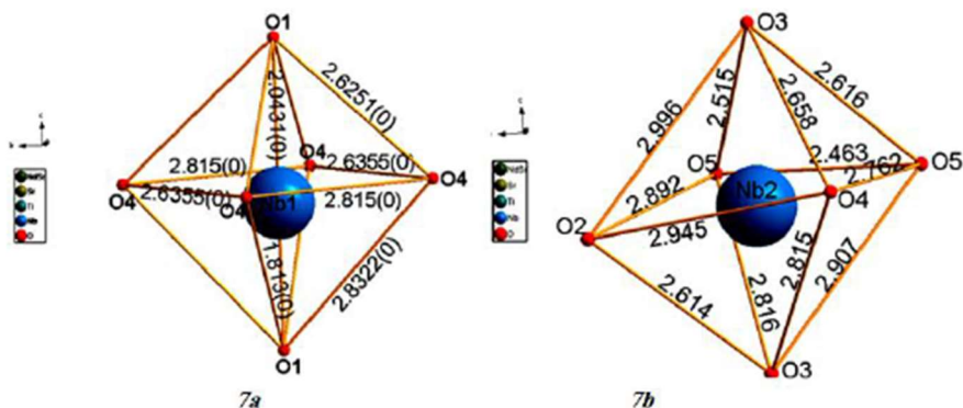
Fig. 7: Polyhedral representations describing the distortions of the distortions of the two kinds of octahedral in \text{Sr}_2\text{Sm}_{1-x}\text{Nd}_x\text{Ti}_2\text{Nb}_3\text{O}_{15}
