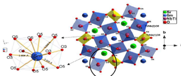
Fig. 6: Projection of the TTB structure on the ab plane with the different sites pentagonal A2, squares A1, and the C triangulars, for a niobate of \text{Sr}_2\text{SmTi}_2\text{Nb}_3\text{O}_{15} formulation
