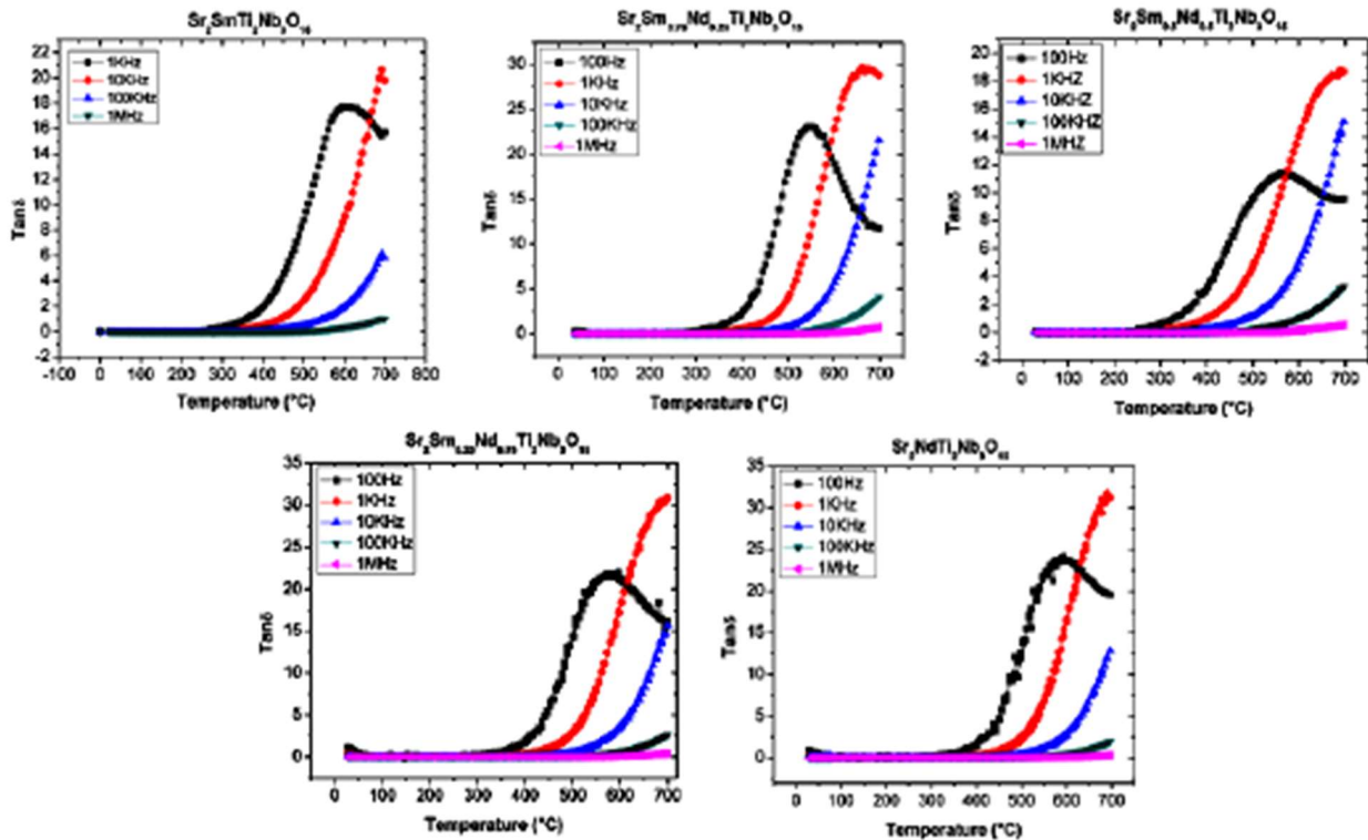
Fig. 9: Thermal evolution of the loss dielectric of Sr_2Sm_{1-x}Nd_xTi_2Nb_3O_{15}
