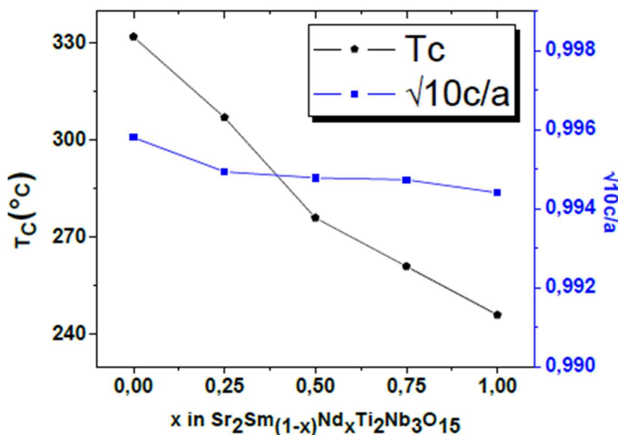
Fig. 5 : Evolution of \frac{c}{a}\sqrt{10} and T c according to the composition for the solid solution Sr 2 Sm (1-x) Nd x Ti 2 Nb 3 O 15 (0 ≤ x ≤ 1)
