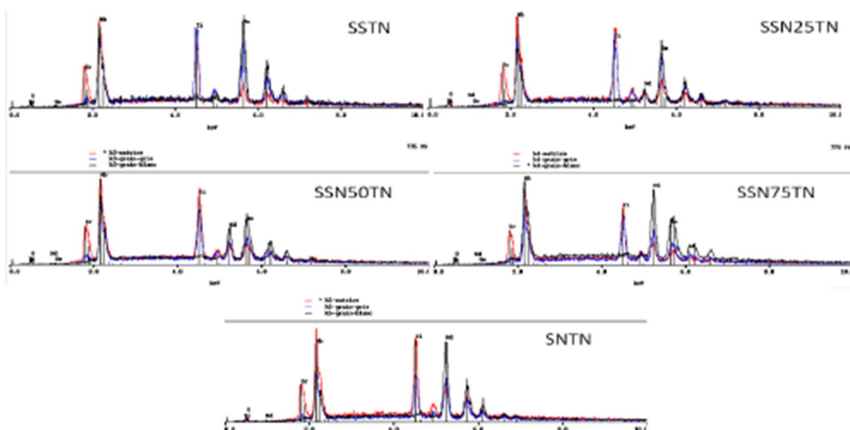
Fig. 11 : Analysis by EDS spectroscopy of the solid solution Sr_2Sm_{(1-x)}Nd_xTi_2Nb_3O_{15}
