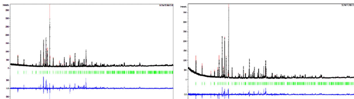
Fig. 3 : Rietveld structural refinement result for \text{Sr}_2\text{SmTi}_2\text{Nb}_3\text{O}_{15} (left) and \text{Sr}_2\text{NdTi}_2\text{Nb}_3\text{O}_{15} (right).
