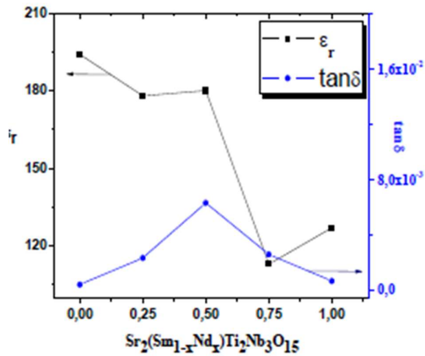
Fig. 10: Variation of \epsilon_r and \tan(\delta) with composition x.
