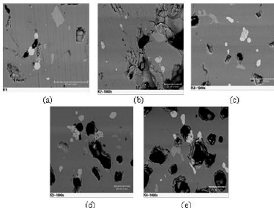
Fig. 12 : SEM analysis of the solid solution \text{Sr}_2\text{Sm}_{(1-x)}\text{Nd}_x\text{Ti}_2\text{Nb}_3\text{O}_{15} (a)=SSTN; (b)=SSN25TN; (c)=SSN50TN; (d)=SSN75TN and (e)=SNTN
