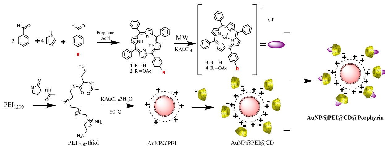
Scheme 1. General pathway of AuNP@PEI@CD@Porphyrin synthesis
