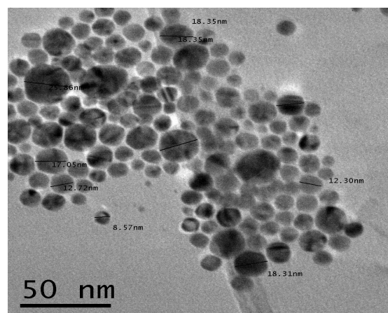
Figure 2: TEM images of gold nanoparticles (AuNP@PEI) with ratio (m PEI /m Au = 0.46)
