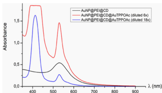
Figure 3: UV-Visible spectra of gold nanoparticles AuNP@PEI@CD alone and with encapsulated gold porphyrin AuTPPOAcCl.
