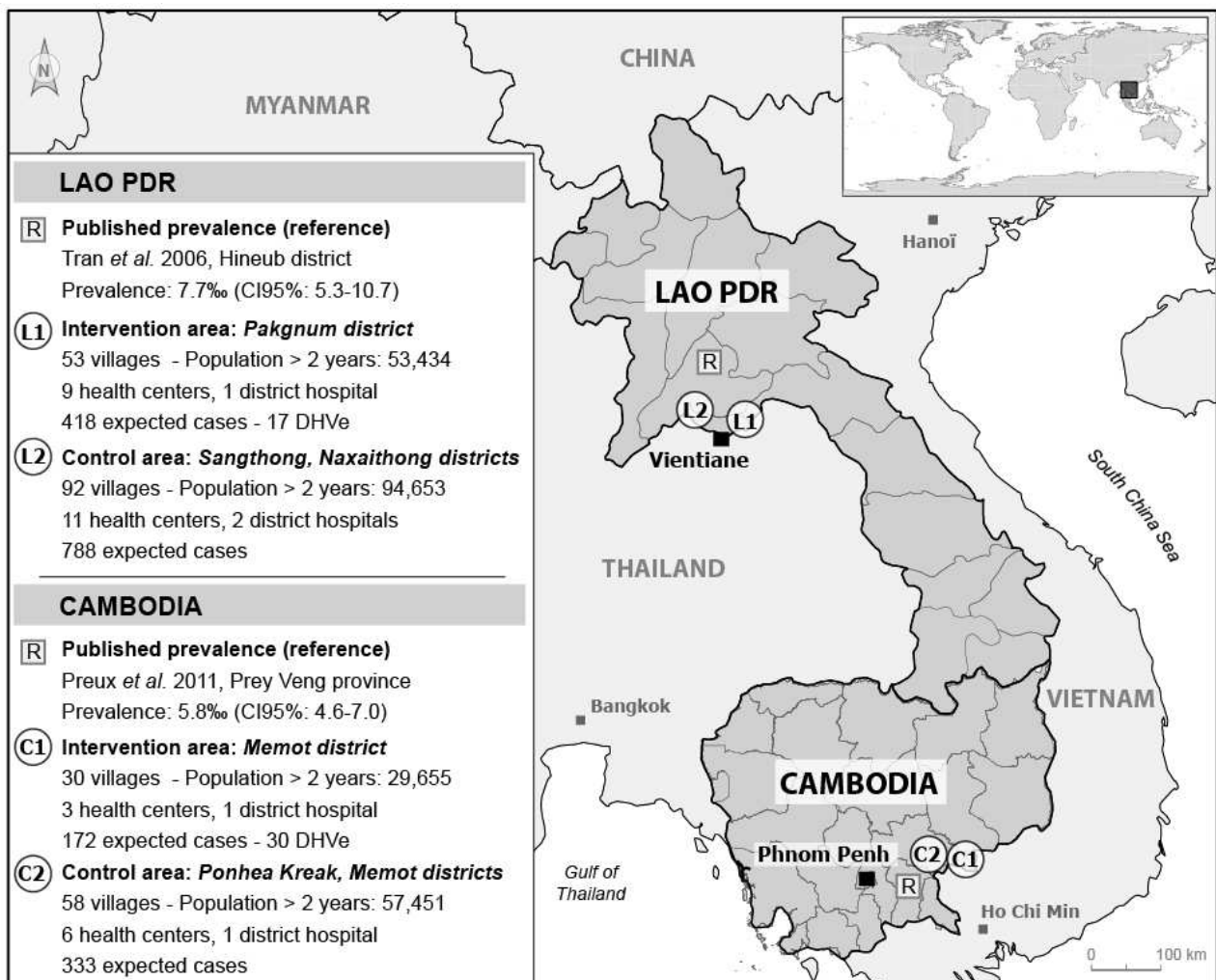
Figure 1. Study areas in Lao PDR and Cambodia ( detailed maps in appendix 4 )
