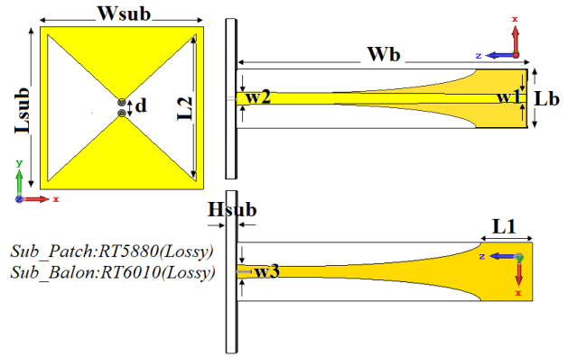
Fig. 2. The proposed matched bowtie antenna with matching balun schematic [13].
