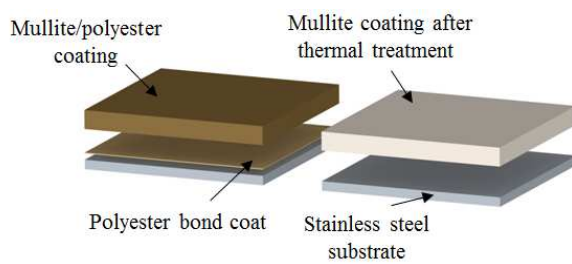
Fig. 8 Approach for getting porous mullite free standing samples with the organic bond coat
