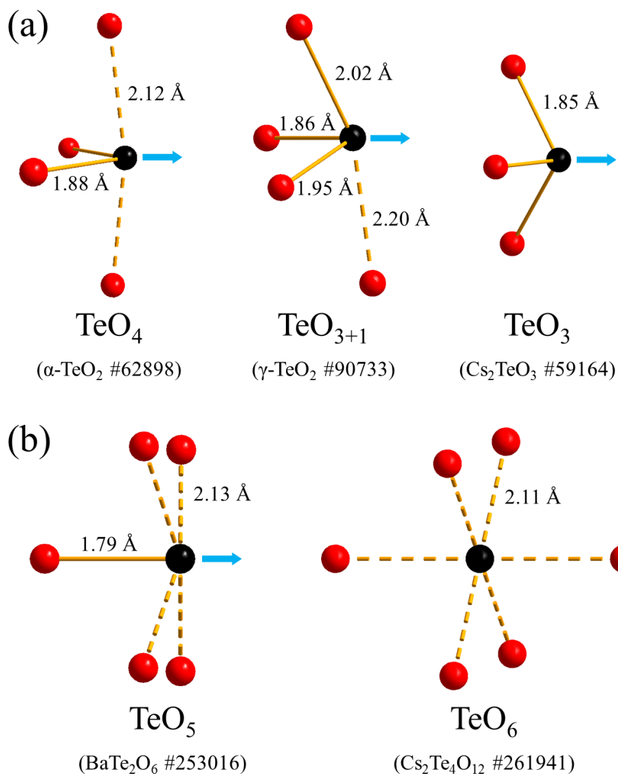
Figure 6. Local environments of Te 4+ cations found in TeO 2 -based crystal structures: (a) usual environments, (b) atypical environments. Te 4+ cores are in black, O 2- anions in red, blue arrows represent Te 4+ LPs and longest Te-O bonds are drawn with dashed lines. Typical compound illustrative of each environment is given in brackets as well as the collection code of its ICSD entry.
