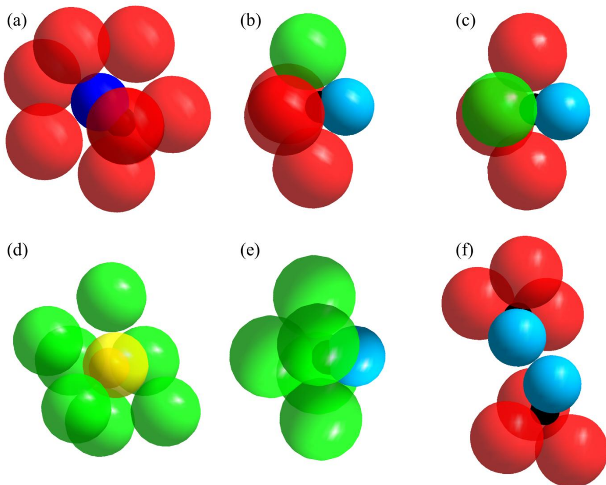
Figure 3 (a, b, c, d and e) for the cases of \alpha -TeO 2 (a), Te 2 O 3 F 2 (b, c) which contains two anion types and PbTeF 6 (d, e) which contains two LP cation types.
