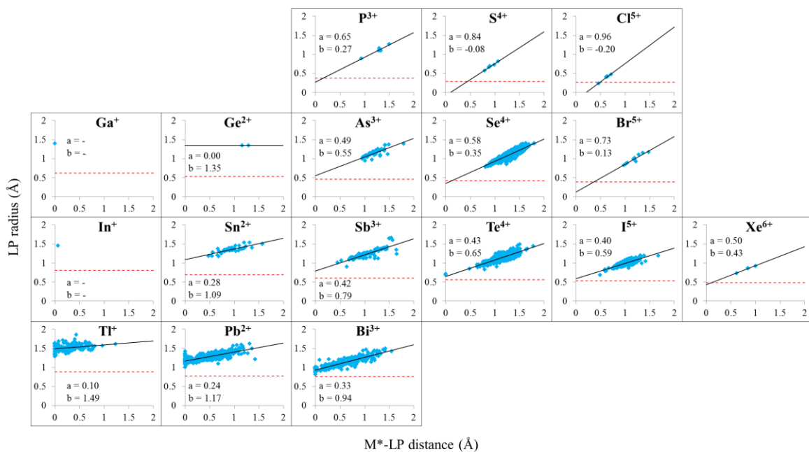
Figure 5. Variation of the LP radius as a function of the M*-LP distance for cations of the p-block elements based on 2380 non-equivalent M* positions in 1138 oxide crystal structures. The dashed red line indicates the core radius value, a and b are the slope and the intercept at the origin of the linear regression (black line) respectively.
