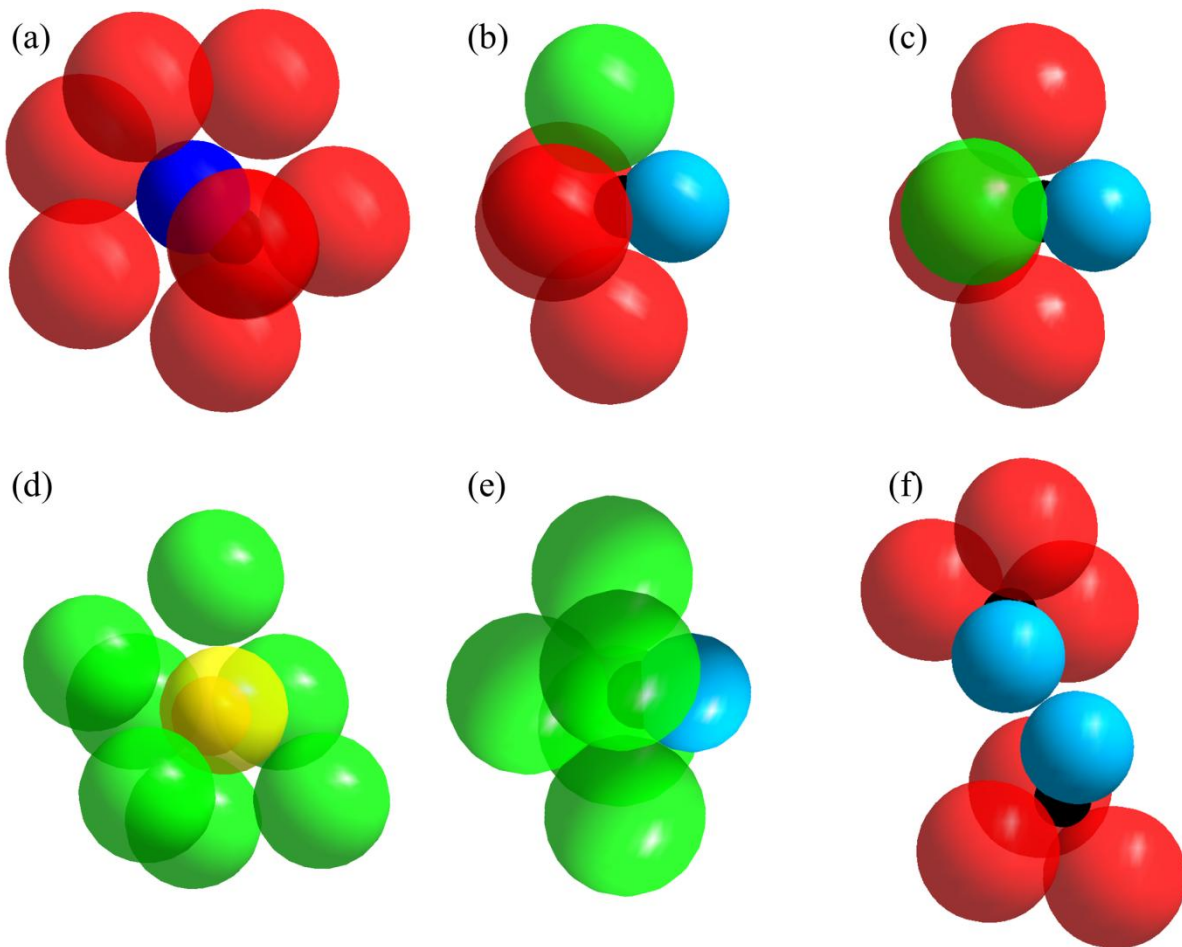
Figure 3. Graphical representations (space-filling model) of the results obtained by applying the present method to LP cations in specific compounds: (a) \text{Te}^{4+} in \alpha\text{-TeO}_2 (ICSD #62898), (b and c) \text{Te}^{4+} (2 different sites) in \text{Te}_2\text{O}_3\text{F}_2 (#82162), (d and e) \text{Pb}^{2+} and \text{Te}^{4+} in \text{PbTeF}_6 (#81865) and (f) \text{Te}^{4+} in \alpha\text{-CdTeO}_3 (#60067). \text{Te}^{4+} cores are in black, \text{Te}^{4+} LPs in blue, \text{Pb}^{2+} core in orange, \text{Pb}^{2+} LP in yellow, \text{O}^{2-} anions in red and \text{F}^- anions in green. Radii of the \text{Te}^{4+} cores, \text{Pb}^{2+} core, \text{O}^{2-} and \text{F}^- anions are 0.56 Å, 0.775 Å, 1.40 Å and 1.33 Å respectively.
