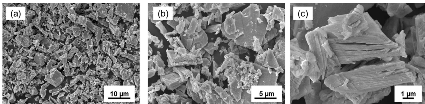
Figure 1. SEM images of the commercial Y_2O_3 powder at different magnifications.
