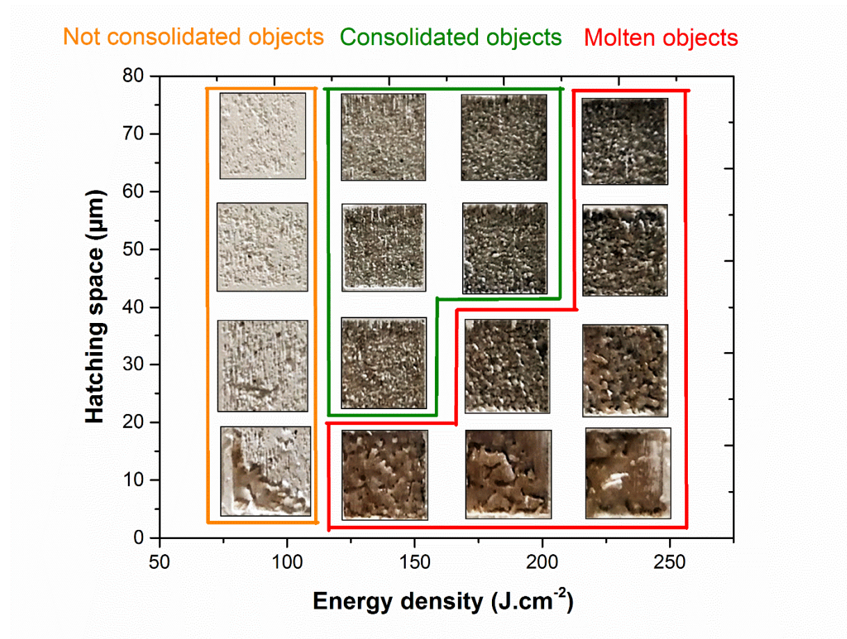
Figure 6. Experimental diagram for the SLS. The color lines separate the samples with acceptable mechanical handling performances from the unconsolidated samples and objects exhibiting significant deformations due to melting.
