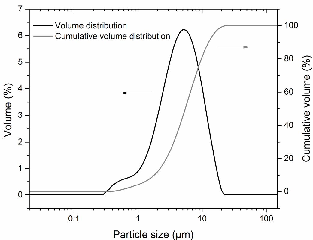
Figure 2. Particle size distribution of the Y_2O_3 commercial powder.
