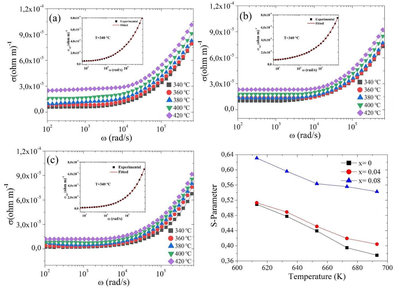
Fig. 11. AC conductivity as a function of frequency at different temperatures for \text{Ba}_5\text{CaTi}_{2-x}\text{Zn}_x\text{Nb}_8\text{O}_{30} ceramics; (a) x=0 , (b) x=0.04 , (c) x=0.08 and (d) variation of the “s” parameter with temperature for \text{Ba}_5\text{CaTi}_{2-x}\text{Zn}_x\text{Nb}_8\text{O}_{30} ceramics.
