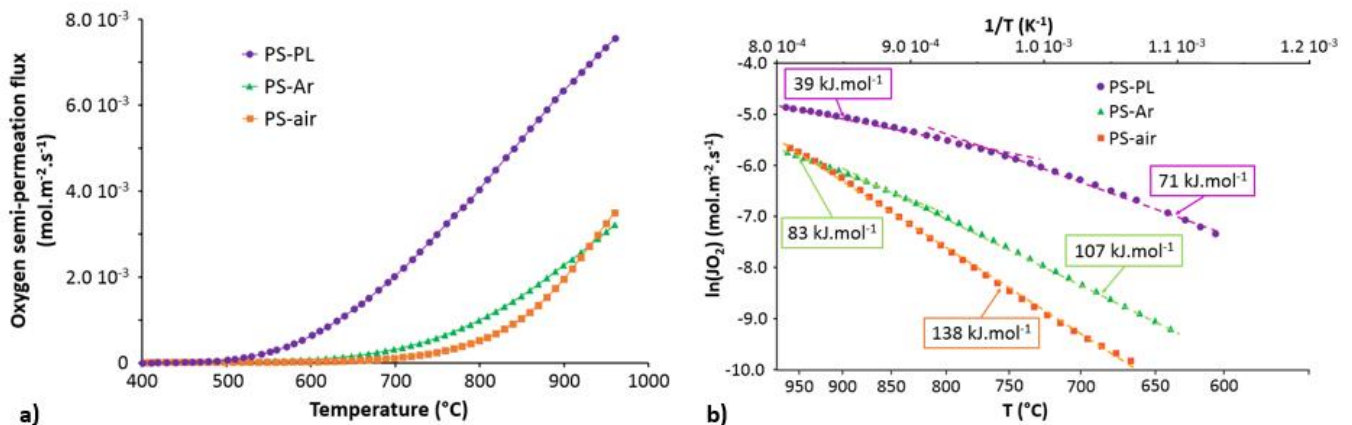
Figure 6: a) Temperature dependence of the oxygen semipermeation fluxes ( J_{O_2} ) through asymmetric membranes under an air ( 100 \text{ ml.min}^{-1} )/argon ( 200 \text{ ml.min}^{-1} ) gradient, b) Arrhenius plots of oxygen fluxes versus 1/T for asymmetric membranes
