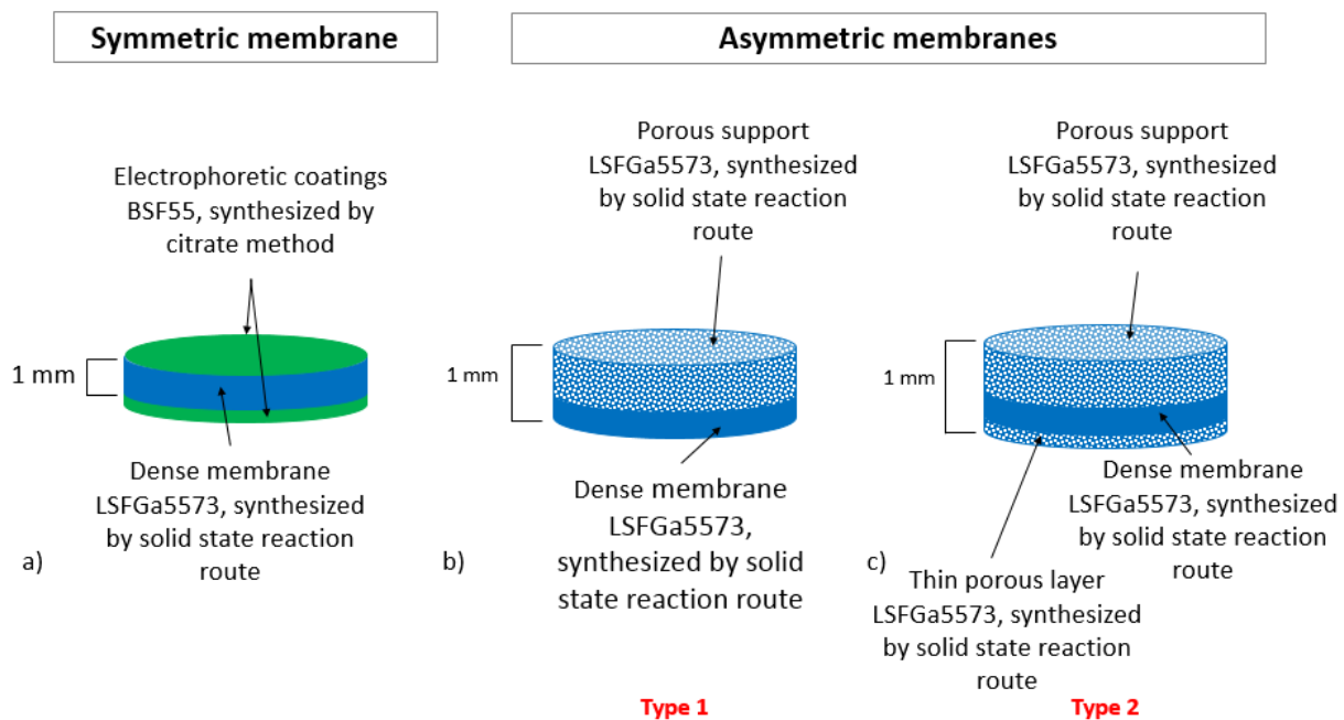
Figure 1: The three studied membrane architectures: symmetric membrane (a), asymmetric membranes without (b), and with thin porous layer (c)
