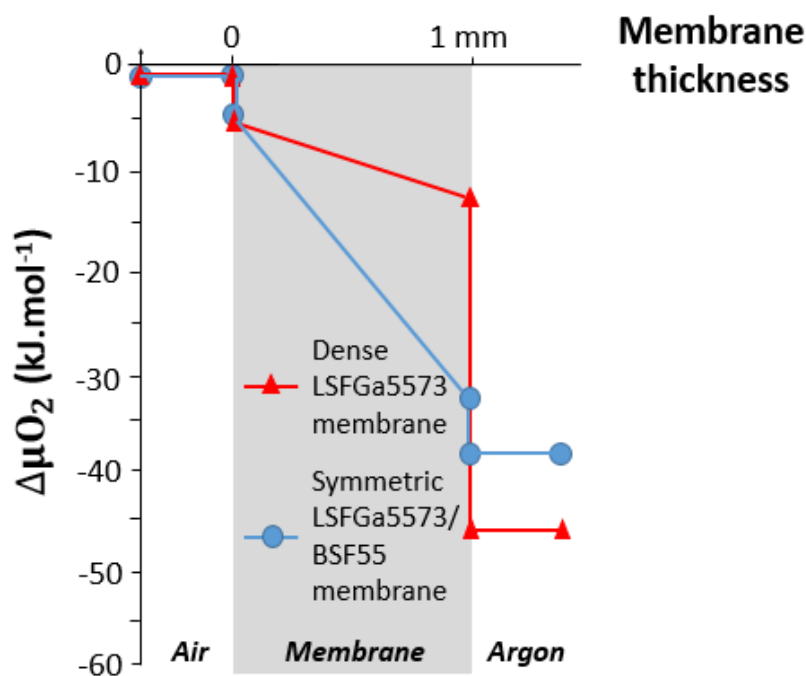
Figure 4: Profiles of the oxygen chemical potential ( \mu_{\text{O}_2} ) through dense LSFGa5573 membrane and symmetric LSFGa5573/BSF55 membrane at 900^\circ\text{C}
