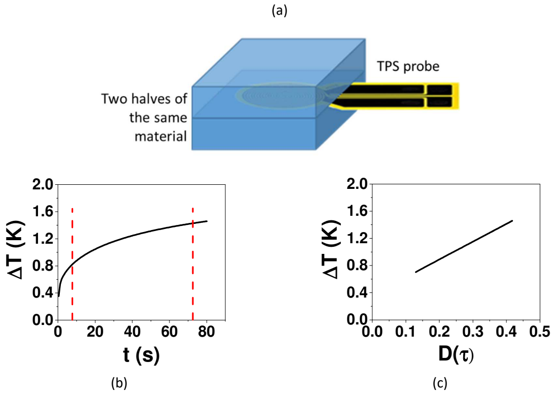
Figure 3: a) Schematic diagram of the hot disk method; b) increase of the temperature as a function of time; c) linear relationship between the temperature increase and the dimensionless specific time function D(\tau) . The dotted lines underline the two limit values: t_{\min} and t_{\max} for the analysis of the thermal conductivity.
