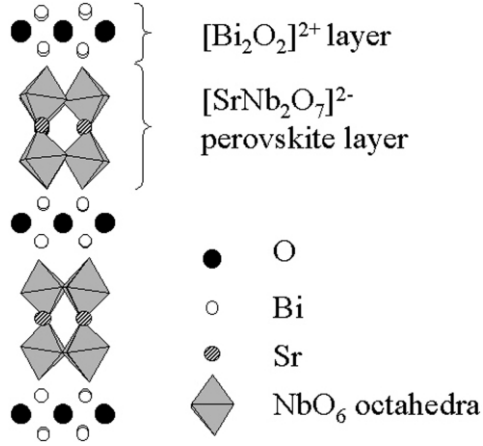
Fig. 1. Projection of \text{SrBi}_2\text{Nb}_2\text{O}_9 oriented along the 0x axis.
