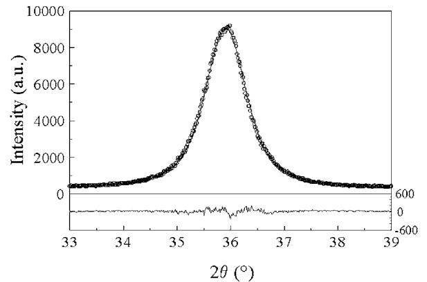
Fig. 3. (0010) Diffraction line reconstructed by means of Eq. (1) of a \text{SrBi}_2\text{Nb}_2\text{O}_9 epitaxial thin film annealed 2 h at 700°C; open circles: observed data points, full line: non-linear least square fit with a Voigt function. The difference line is shown with a separate scale.
