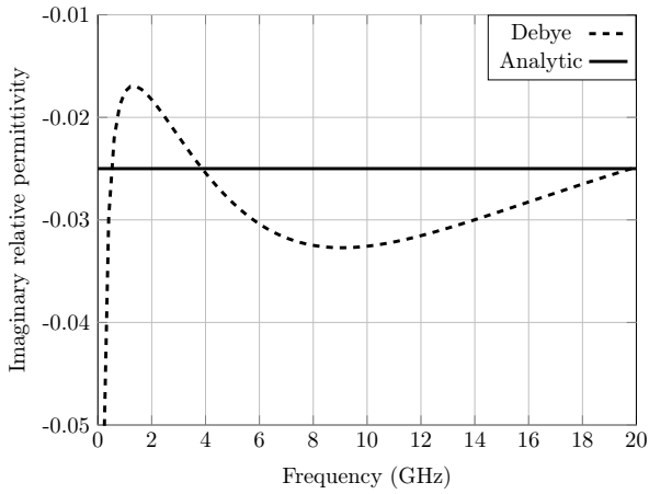
Fig. 2. Imaginary part of the FR4 Debye relative permittivity compared with theory.
