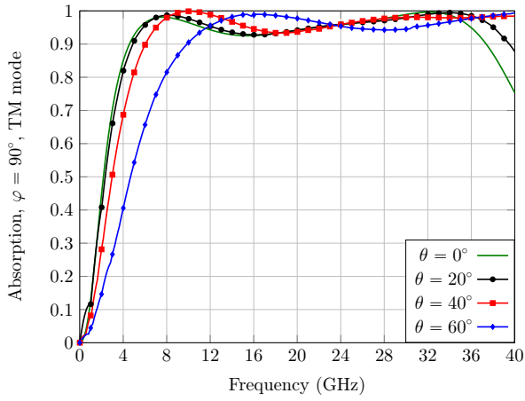
Fig. 5. TM mode absorption curve for the PMI/PET absorber.
