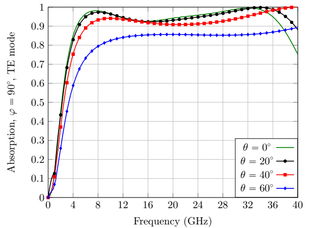
Fig. 4. TE mode absorption curve for the PMI/ PET absorber.
