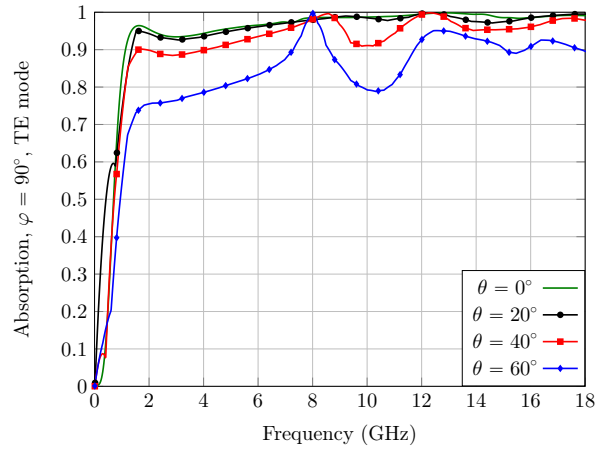
Fig. 7. TE mode absorption curve for the FR4/ITO absorber.
