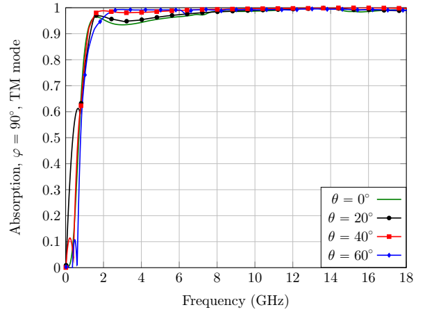
Fig. 8. TM mode absorption curve for the FR4/ITO absorber.
