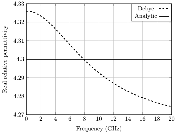
Fig. 1. Real part of the FR4 Debye relative permittivity compared with theory.
