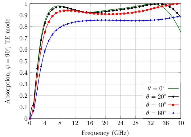
Fig. 4. TE mode absorption curve for the PMI/ PET absorber.
