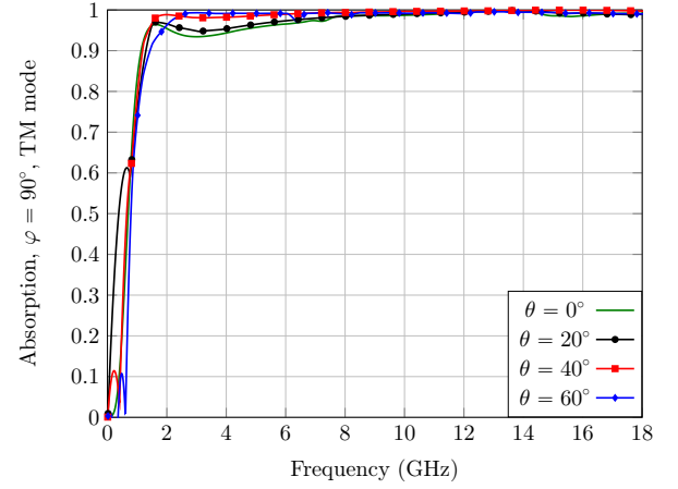
Fig. 8. TM mode absorption curve for the FR4/ITO absorber.
