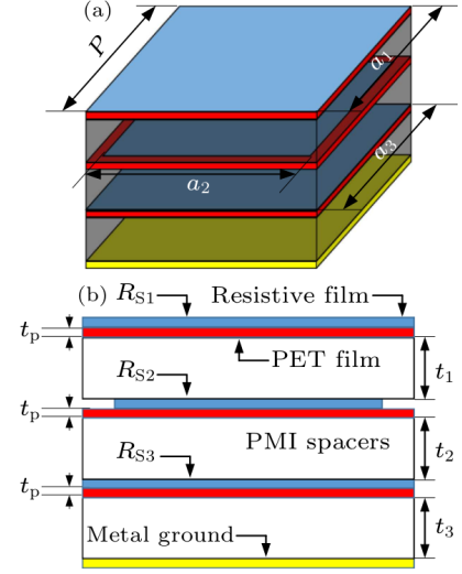
Fig. 3. Pattern geometry of the PMI (white) and PET (red) absorber with resistive films (blue) [7]. t_1 = 2 mm, t_2 = 4 mm, t_3 = 3 mm, t_p = 0.175 mm, P = a_1 = a_3 = 14 mm, a_2 = 12.5 mm.
