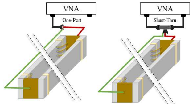
Fig. 5. Measurement setups.
