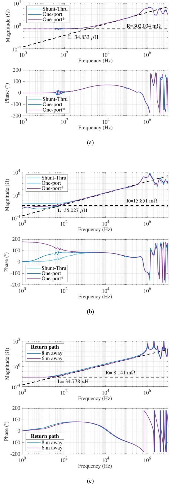
Fig. 7. Impedance of the reinforced concrete duct. (a) Measured in C1. (b) Measured in C2. (c) Calculated using TEMSI-FD.
