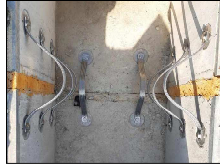
Fig. 3. Interconnection of two sections of the concrete duct.
