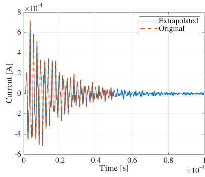
Fig. 5. Extrapolation of the current in segment S1 of the auxiliary wire.
