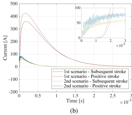
Fig. 11. Currents in segment S1 in the worst-case scenarios. (a) Insulated wire. (b) Auxiliary wire.
