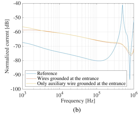
Fig. 7. Normalized currents in segment S1 when the wires are grounded at the entrance to the buildings. (a) Insulated wire. (b) Auxiliary wire.
