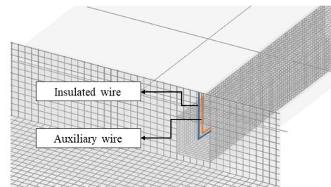
Fig. 4. Position of the wires inside the reinforced concrete duct.
