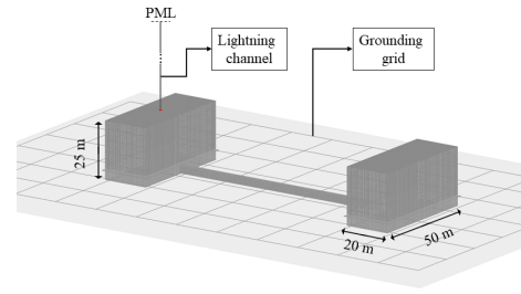
Fig. 1. Calculation model of the reference case.
