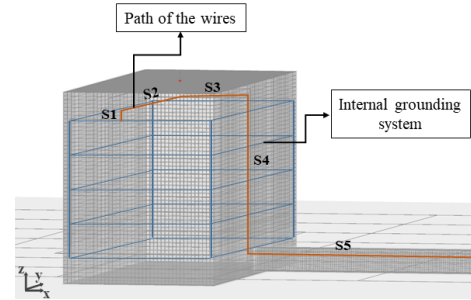
Fig. 3. Detailed view of the first building in the reference case.
