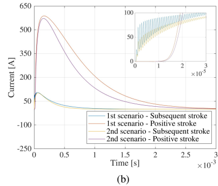
Fig. 12. Currents in segment S1 in the worst-case scenarios when the wires are grounded at the entrance to the buildings. (a) Insulated wire. (b) Auxiliary wire.
