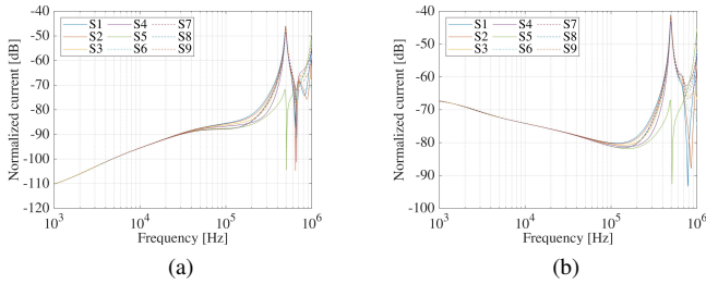
Fig. 6. Normalized currents in the reference case. (a) Insulated wire. (b) Auxiliary wire.
