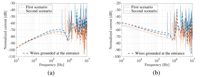
Fig. 10. Normalized currents in segment S1 in the worst-case scenarios. (a) Insulated wire. (b) Auxiliary wire.
