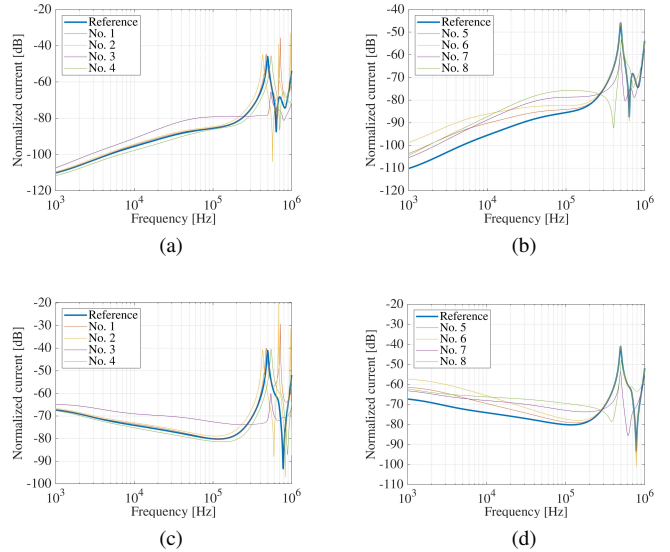
Fig. 8. Cases in which the highest normalized currents are observed in segment S1. (a) Insulated wire, cases 1 to 4. (b) Insulated wire, cases 5 to 8. (c) Auxiliary wire, cases 1 to 4. (d) Auxiliary wire, cases 5 to 8.
