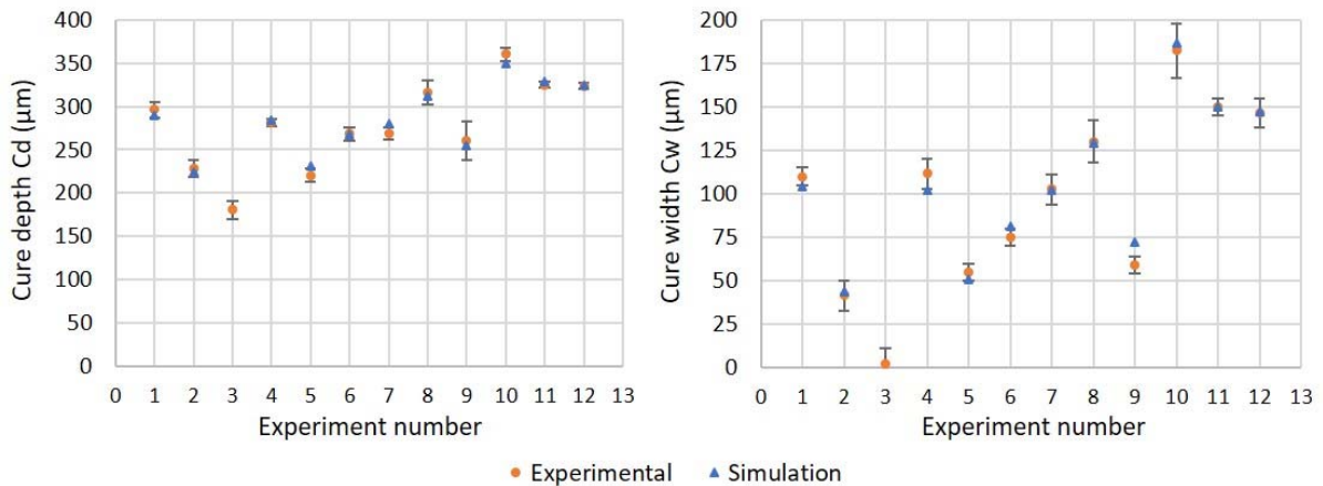
Fig. 10. Comparison between experimental and simulated cure depths Cd and cure widths Cw
