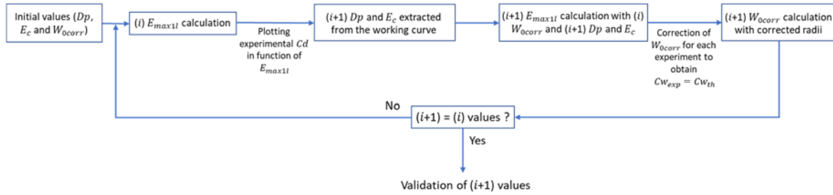
Fig. 6. Process for Dp and E_c determination
