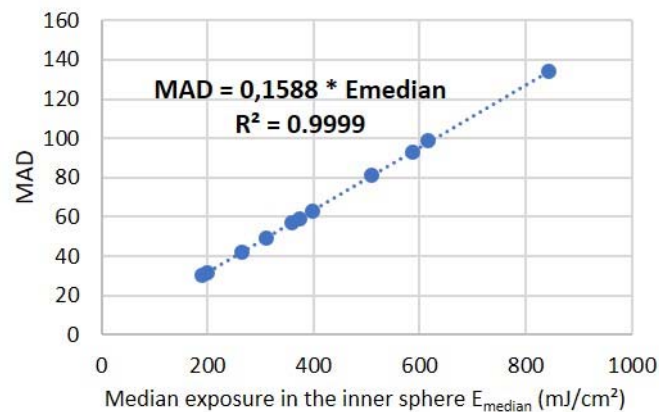
Fig. 19. MAD factor in function of the median exposure in the inner sphere of a 10-layer part, for each set of parameters except E3.
