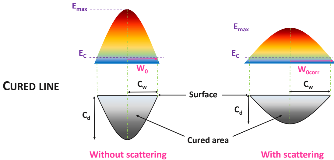
Fig. 3. Influence of particles in suspension on the light scattering, exposure distribution and cured area [14]
