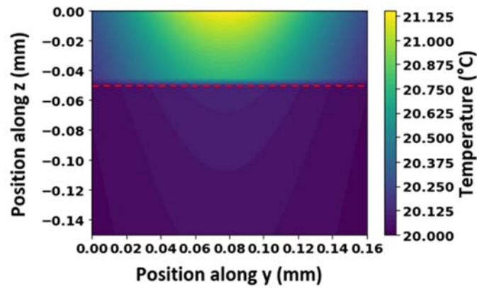
Fig. 18. Temperature discontinuity at the interface between 2 layers at the end of a single pulse. This pulse targets the top surface of a 2 layer-part printed with E1 parameters. The bottom layer (under the red dotted line) is already insulated and polymerized, while the top layer receives its first pulse.
