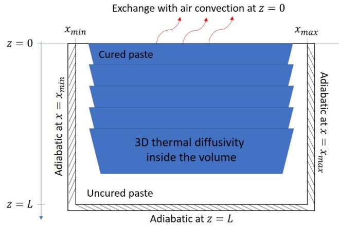
Fig. 5. Summary of different thermal exchanges and limit conditions considered in the simulation.
