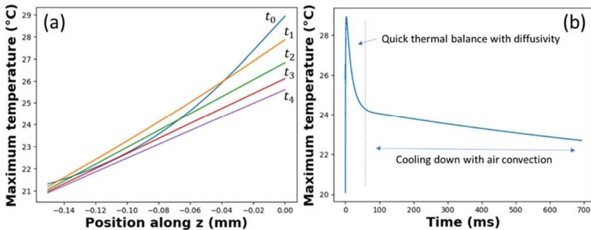
Fig. 16. Evolution of the maximum internal temperature (a) after the last pulse, in function of the depth and for different times ( t_0 - t_4 ) and (b) in the whole part, in function of the time during and after laser exposure. In the left graph, each curve is separated by about 3ms, and t_0 corresponds to the moment the last pulse ends.
