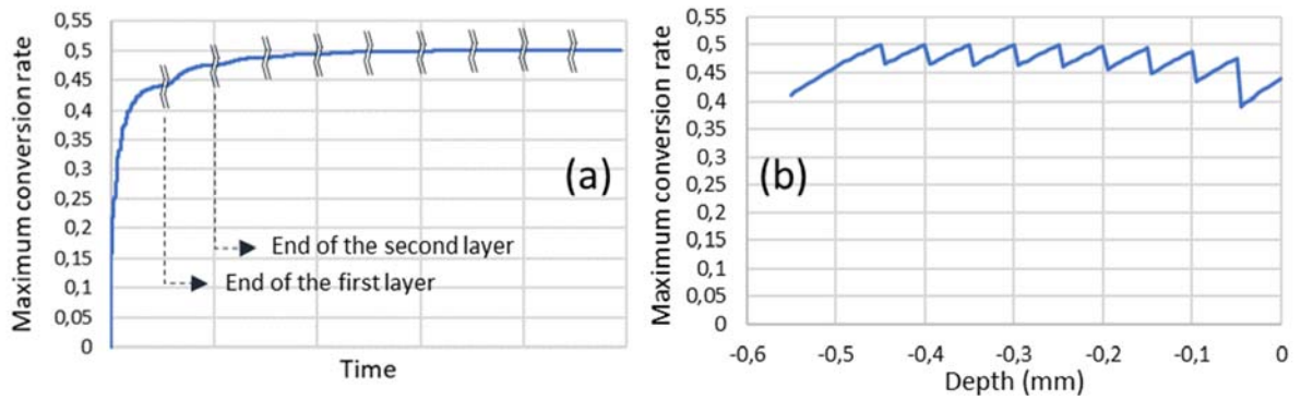
Fig. 14. Evolution of the maximum conversion rate in function of (a) the time of printing and (b) the depth, on a 10-layer part manufactured with E1 parameters. The depth 0mm corresponds to the top surface of the part. Time is not displayed because of discontinuity between layers due to stereolithography process. Transition from one layer to another (~30s) is here considered instant to help observation.
