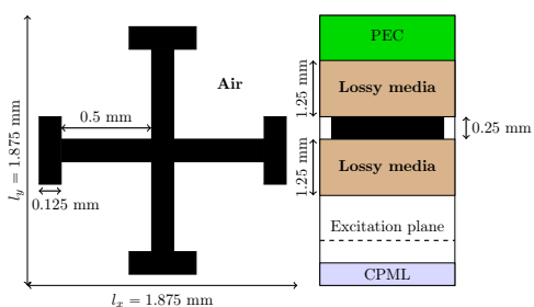
Figure 2: Elementary pattern geometry. CPML absorbing condition are used to deal with outgoing waves.
